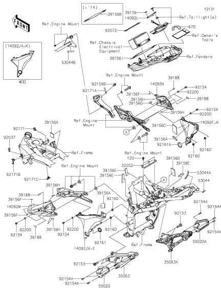
E-6 Frame Fittings(2/2)
