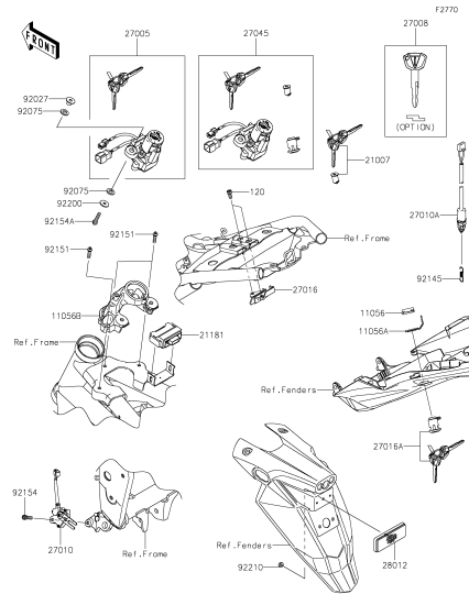
G-13 Ignition Switch
