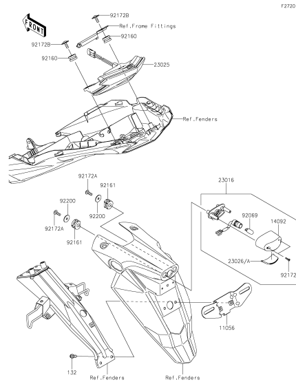
G-10 Taillight(s)
