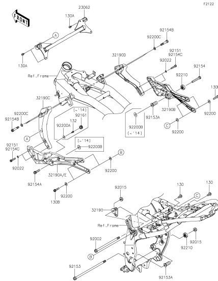
E-4 Engine Mount
