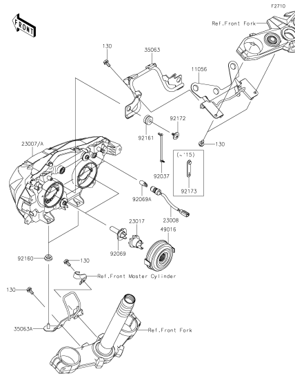
G-9 Headlight(s)
