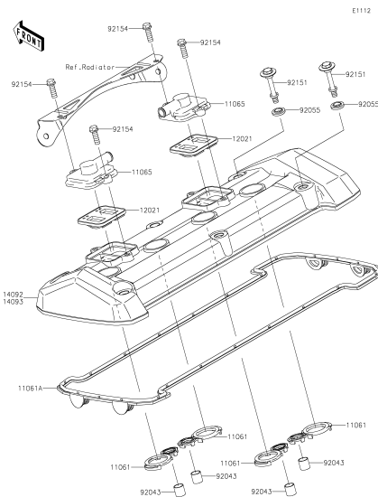
B-4 Cylinder Head Cover
