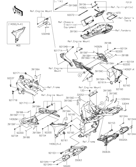
E-5 Frame Fittings(1/2)
