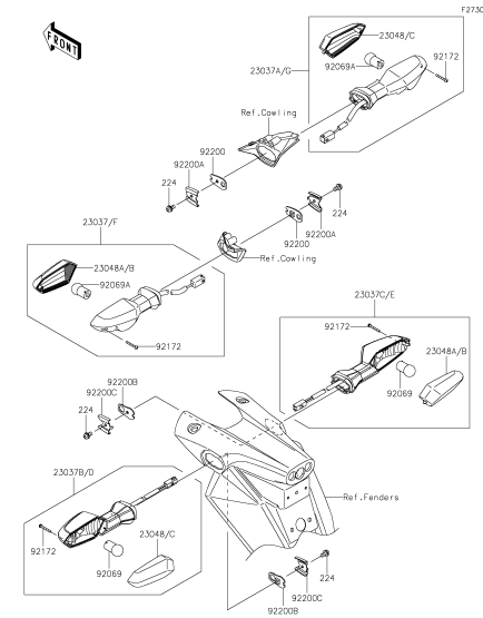
G-11 Turn Signals
