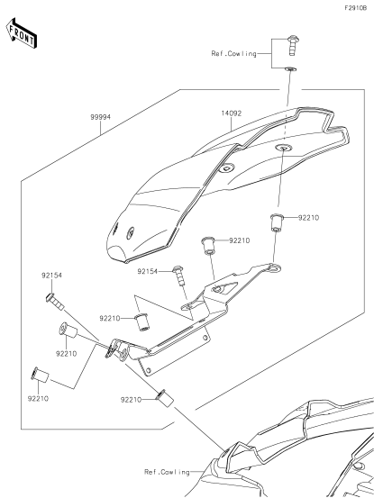
I-9 Accessory(Meter Cover)
