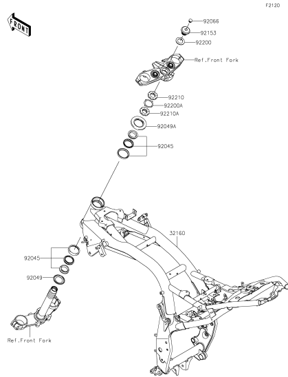
E-3 Frame
