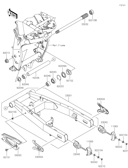
E-7 Swingarm
