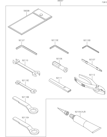
G-14 Owner's Tools
