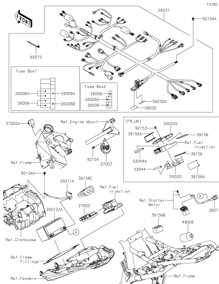
G-12 Chassis Electrical Equipment
