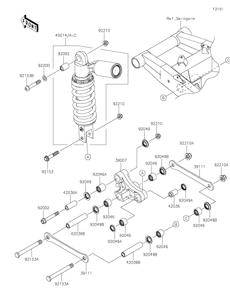
E-8 Suspension/Shock Absorber
