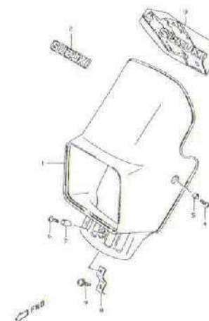
FIG.37 HEADLAMP COVER (MODEL R/S/T) (G-5)
