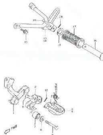
FIG.32 FOOTREST (F-6)
