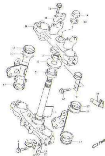
FIG.46 STEERING STEM (I-2)
