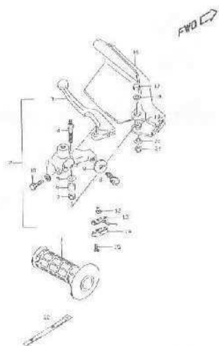
FIG.41A LEFT HANDLE LEVER (MODEL V/W) (G-12)
