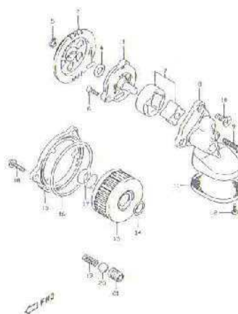
FIG.13 OIL PUMP (C-8)
