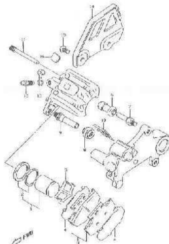
FIG.54 REAR CALIPER (I-12)
