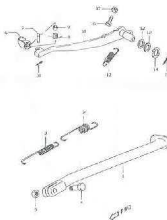
FIG.31 STAND - REAR BRAKE (F-5)
