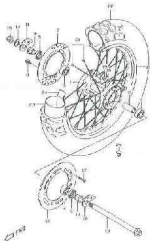
FIG.53A REAR WHEEL (MODEL T/V/W) (I-11)
