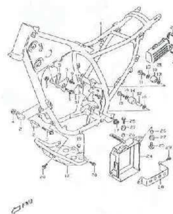
FIG.33 REAR GLIP (F-7)
