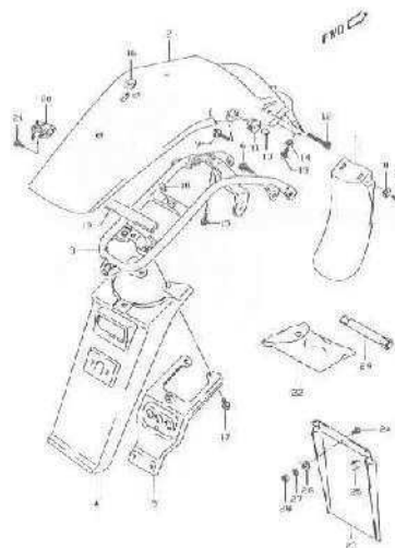
FIG.42 REAR FENDER (H-2)
