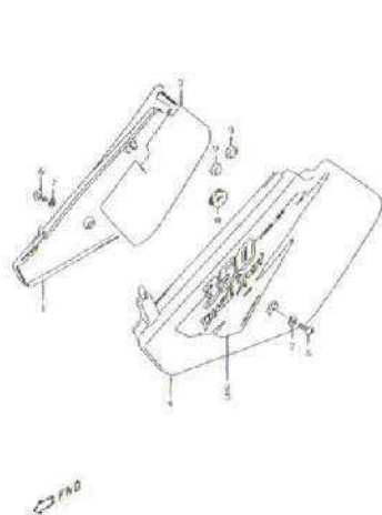
FIG.36A FRAME COVER (MODEL T) (G-3)
