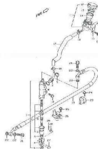
FIG.55 REAR MASTER CYLINDER (I-13)
