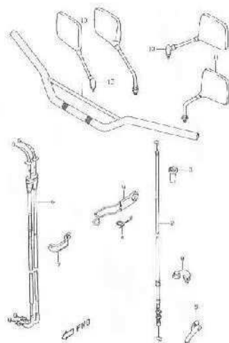
FIG.39 HANDLEBAR (G-8)
