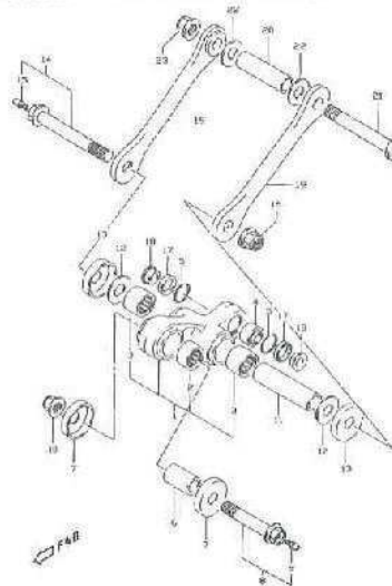
FIG.52 REAR CUSHION LEVER (I-8)
