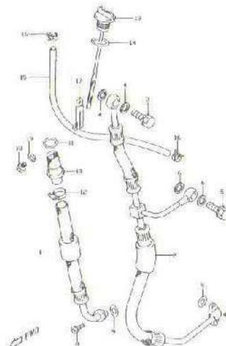
FIG.14 OIL HOSE (C-9)
