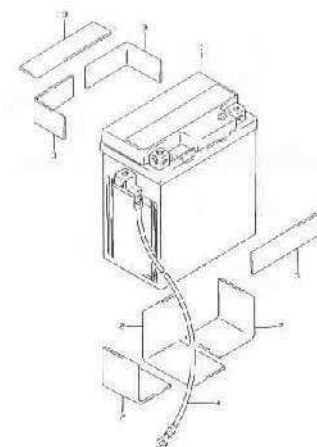
FIG.22 BATTERY (E-2)
