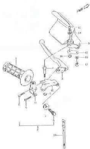
FIG.41 LEFT HANDLE LEVER (MODEL R/S/T) (G-11)
