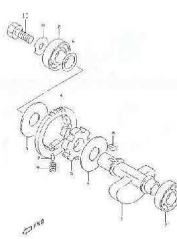
FIG.7 CRANK BALANCER (B-9)
