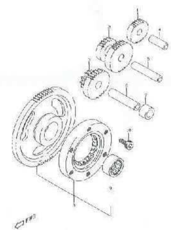
FIG.6 STARTER CLUTCH (B-8)
