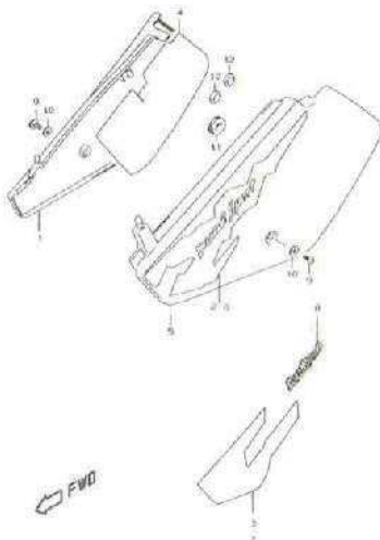
FIG.36B FRAME COVER (MODEL V/W) (G-4)
