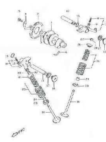
FIG.8 CAM SHAFT - VALVE (B-10)
