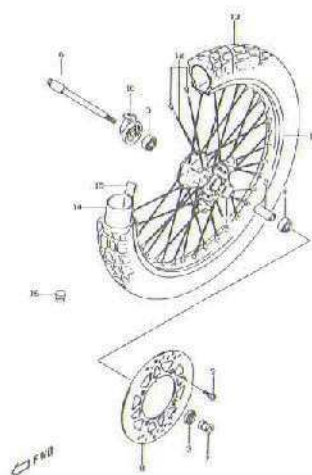
FIG.47 FRONT WHEEL (I-3)
