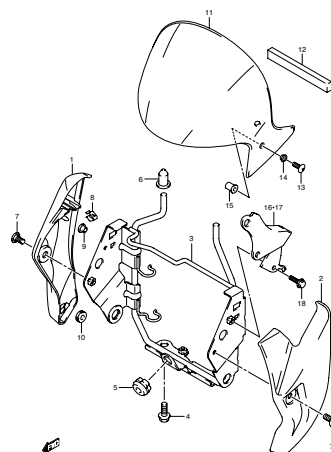
FIG.43C HEADLAMP COVER (MODEL L0) (1-G-3)
