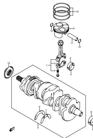
FIG.7 CRANKSHAFT (1-B-11)
