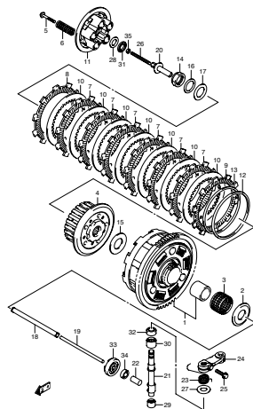
FIG.21 CLUTCH (1-C-14)
