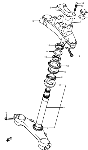
FIG.52 STEERING STEM (GSR600K6/K7) (1-H-6)
