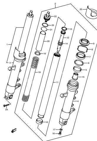
FIG.51A FRONT DAMPER (GSR600AK8/AK9/AL0) (1-H-5)
