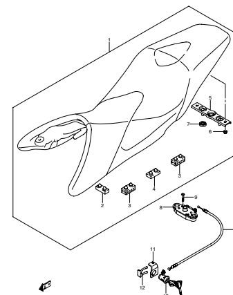
FIG.49 SEAT (1-G-12)
