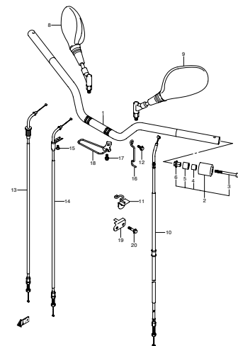
FIG.45 HANDLEBAR (1-G-8)
