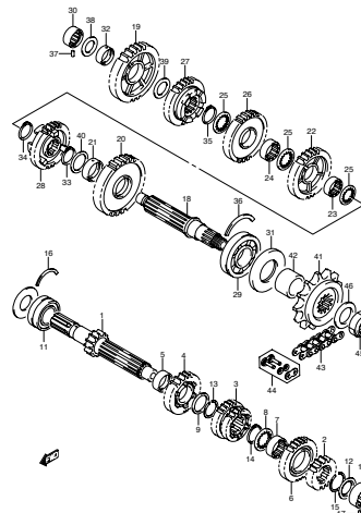
FIG.22 TRANSMISSION (1-D-2)
