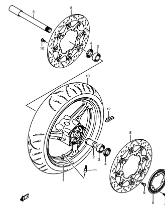
FIG.53A FRONT WHEEL (GSR600AK7/AK8/AK9) (1-H-9)
