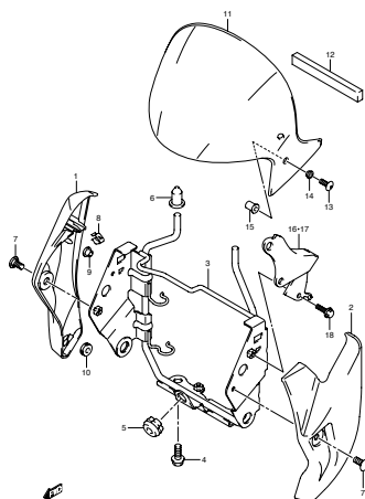
FIG.43B HEADLAMP COVER (MODEL K9) (1-G-2)
