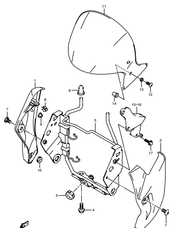
FIG.43A HEADLAMP COVER (MODEL K8) (1-F-15)
