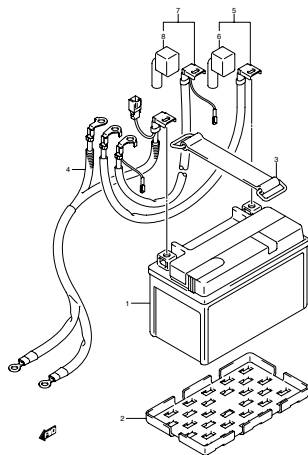
FIG.27 BATTERY (1-D-10)
