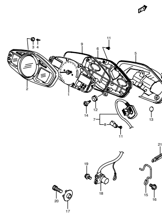
FIG.29A SPEEDOMETER (GSR600AK7/AK8) (1-D-13)
