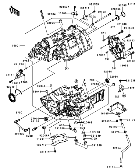
C-5 Crankcase(2/2)(~ER650AE057323)
