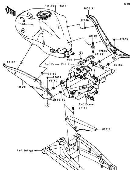
G-4 Side Covers/Chain Cover
