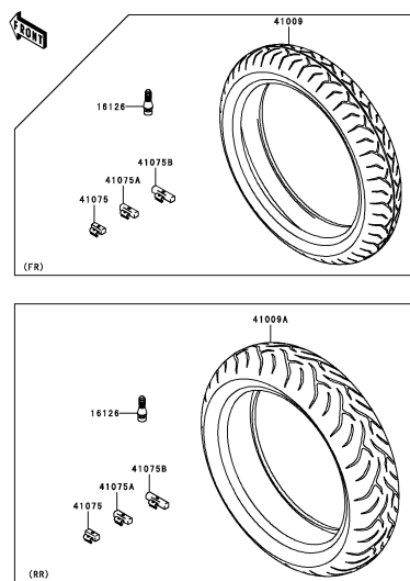
E-13 Tires
