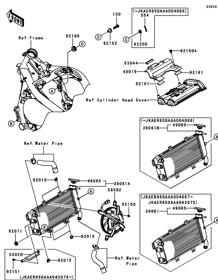
D-9 Radiator
