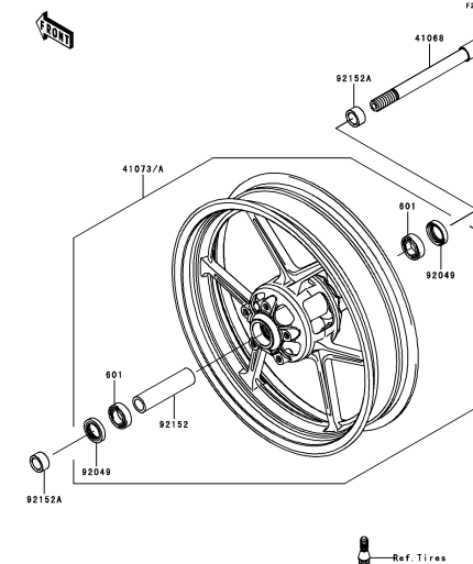
E-14 Front Hub
