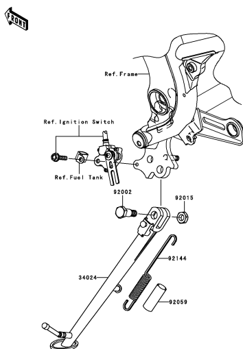
E-12 Stand(s)
