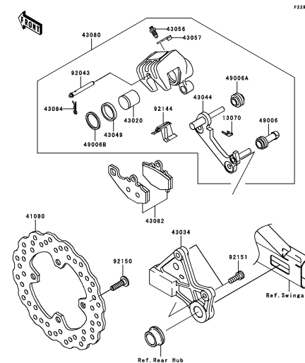
F-8 Rear Brake
