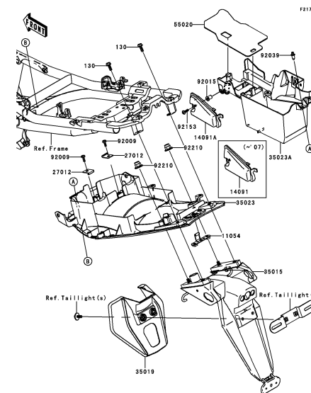
E-11 Rear Fender(s)
