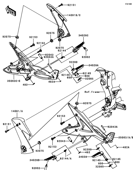
E-9 Footrests
