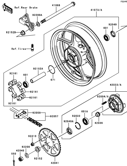
F-3 Rear Hub
