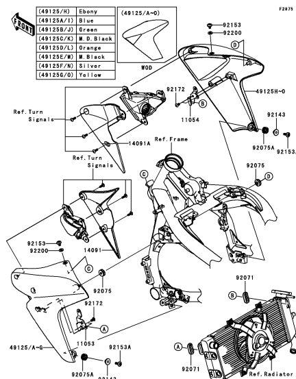
H-10 Shroud
