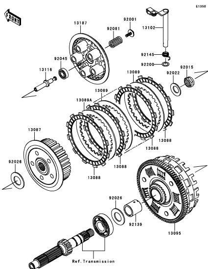
B-12 Clutch
