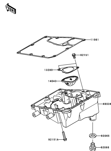
C-11 Oil Pan
