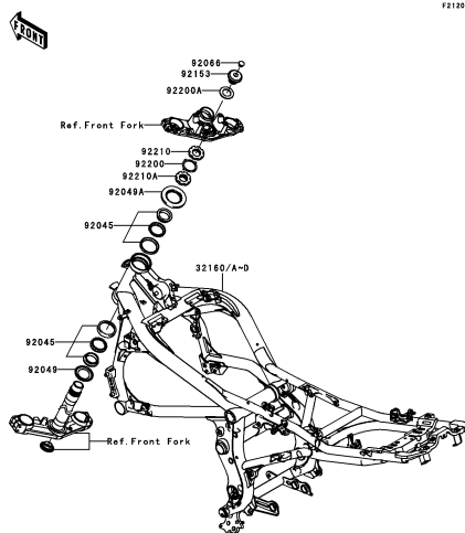
E-3 Frame
