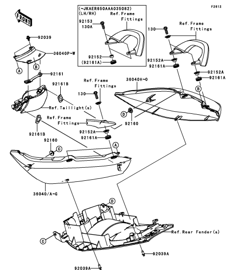
G-5 Seat Cover
