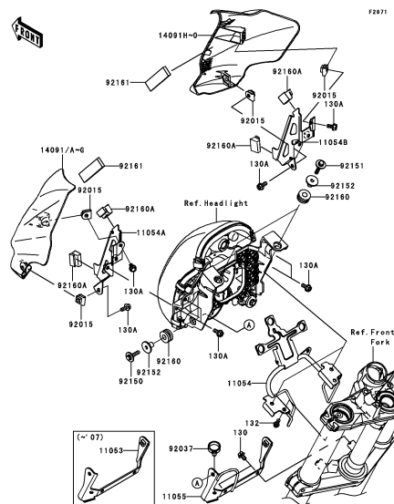
H-9 Cowling
