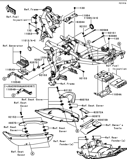
E-6 Frame tings(JKAER650AAA035083~)
