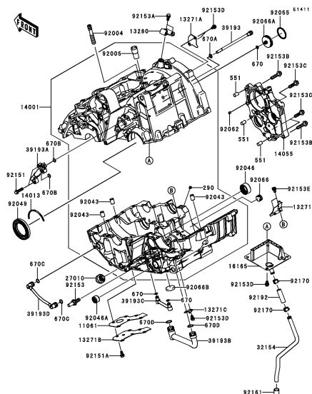
C-4 Crankcase(1/2)(~ER650AE057323)
