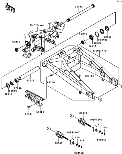
E-7 Swingarm
