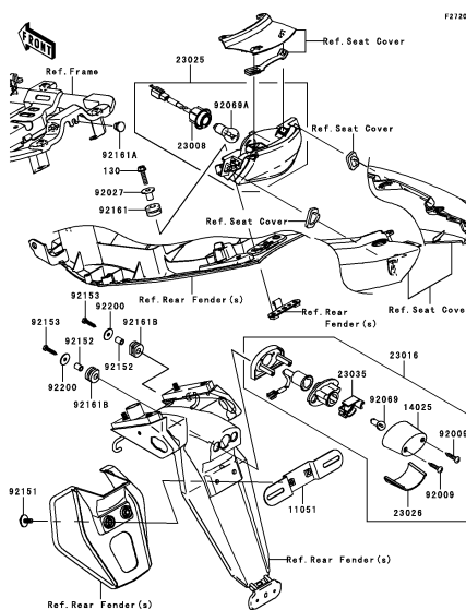
G-7 Taillight(s)
