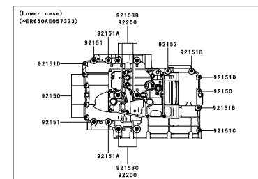
C-8 Crankcase Bolt Pattern
