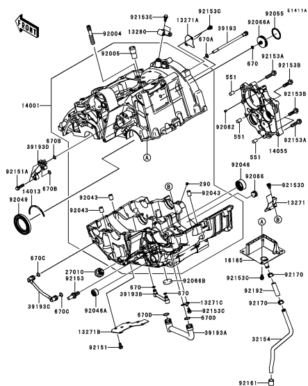
C-6 Crankcase(1/2)(ER650AE057324~)
