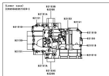
C-9 Crankcase Bolt Pattern
