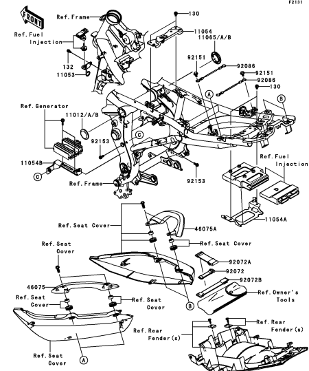
E-5 Frame fittings(~JKAER650AAA035082)
