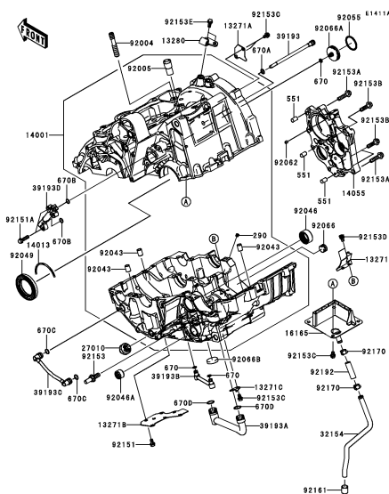
C-7 Crankcase(2/2)(ER650AE057324~)
