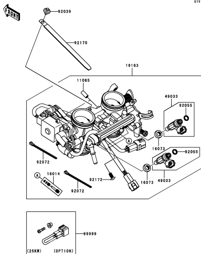
C-12 Throttle
