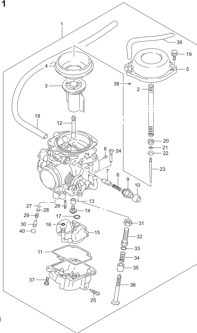
FIG.11 (C-3) CARBURETOR
