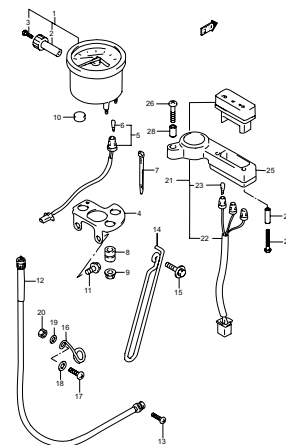
FIG.24 SPEEDOMETER (D-6)
