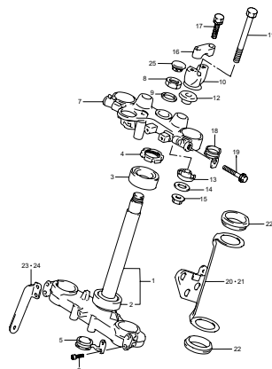
FIG.45 STEERING STEM (H-4)
