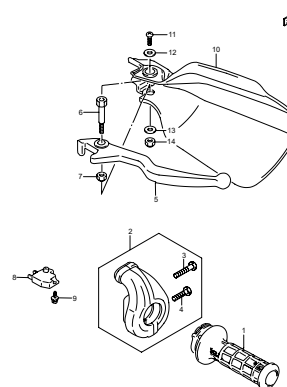
FIG.39 RIGHT HANDLE LEVER (G-5)
