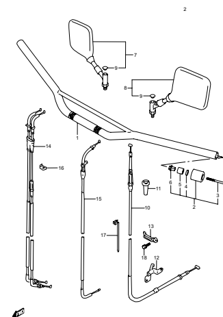
FIG.38 HANDLEBAR (G-4)
