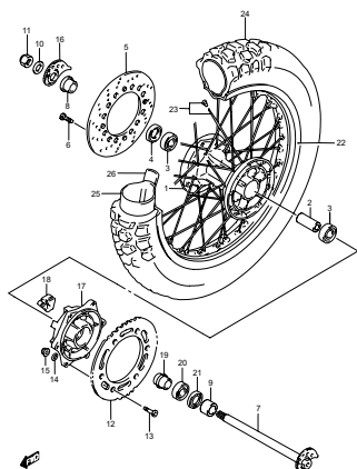
FIG.51A REAR WHEEL (MODEL K8/K9/L0) (H-11)
