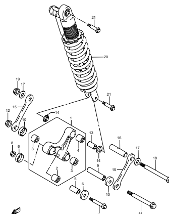
FIG.50 REAR CUSHION LEVER (H-9)
