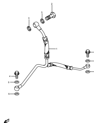
FIG.16 OIL PIPE (C-8)
