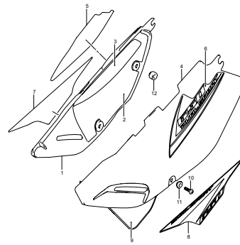
FIG.36A FRAME COVER (MODEL K8/K9/L0) (F-8)
