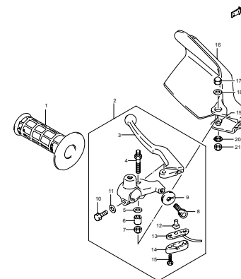
FIG.39A LEFT HANDLE LEVER (MODEL K6/K7/ K8/K9) (G-6)
