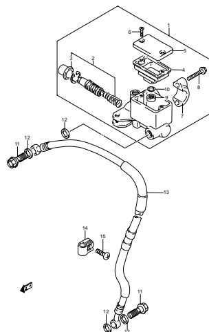
FIG.48 FRONT MASTER CYLINDER (H-7)
