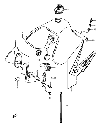
FIG.34B FUEL TANK (MODEL L0) (F-4)
