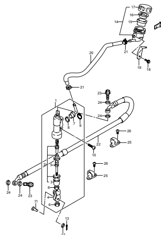
FIG.54 REAR MASTER CYLINDER (H-13)
