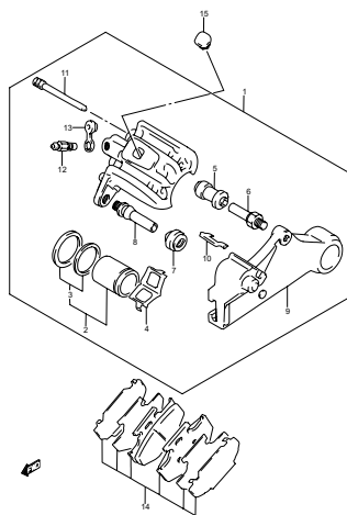
FIG.53 REAR CALIPER (H-12)
