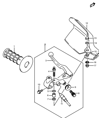
FIG.39B LEFT HANDLE LEVER (MODEL L0) (G-7)
