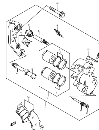
FIG.47 FRONT CALIPER (H-6)
