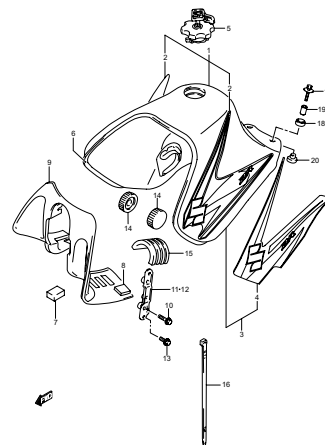
FIG.36A FRAME COVER (MODEL K8/K9/L0) (F-8)
