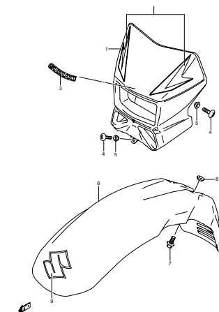
FIG.37A HEADLAMP HOUSING (MODEL K9/ L0) (G-3)
