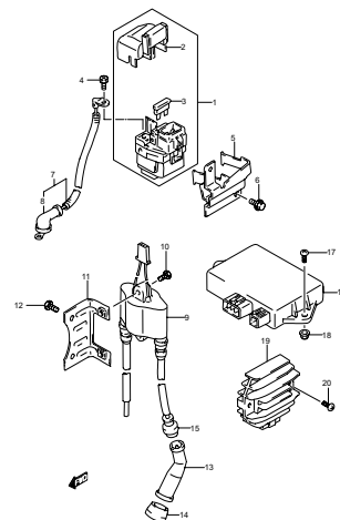
FIG.23 ELECTRICAL (D-5)
