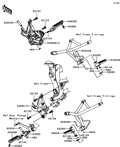
E-9 Footrests
