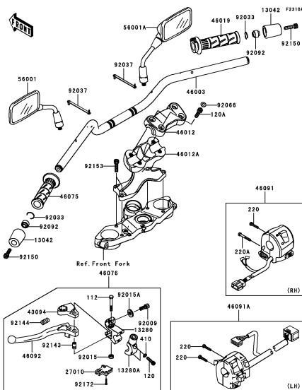
F-12 Handlebar(A9F)
