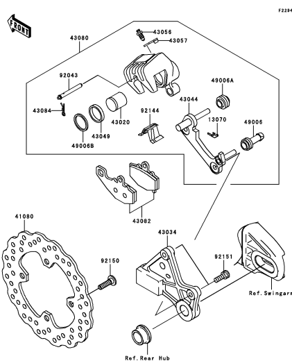
F-10 Rear Brake
