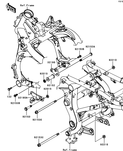
E-5 Engine Mount
