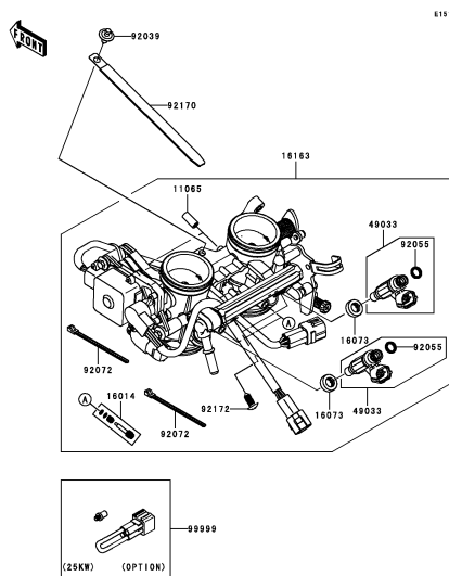
C-12 Throttle
