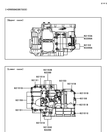
C-5 Crankcase(2/2)(~ER650AE057323)
