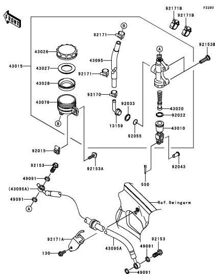
F-9 Rear Master Cylinder
