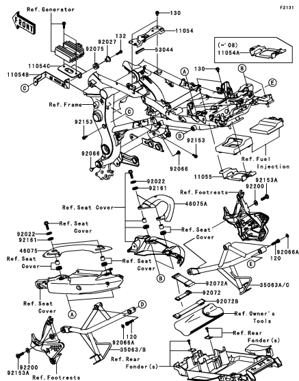
E-6 Frame Fittings
