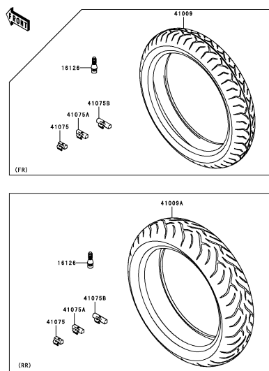
E-13 Tires
