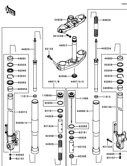
F-13 Front Fork
