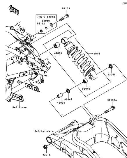
E-8 Suspension/Shock Absorber
