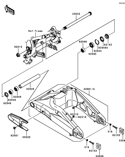
E-7 Swingarm
