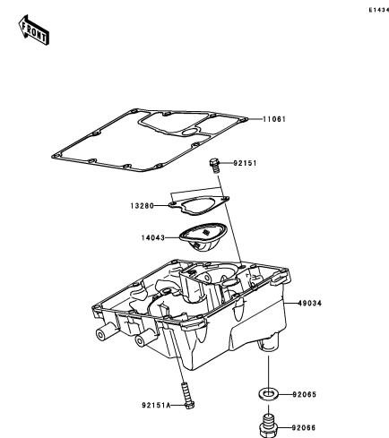
C-11 Oil Pan
