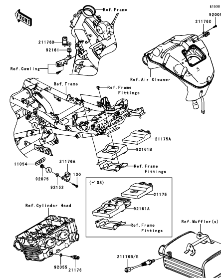
C-14 Fuel Injection
