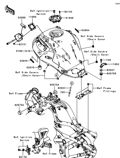
F-14 Fuel Tank(A7F/A8F)
