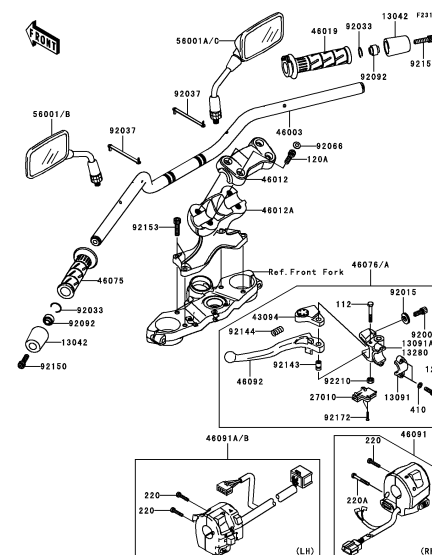
F-11 Handlebar(A7F/A8F)
