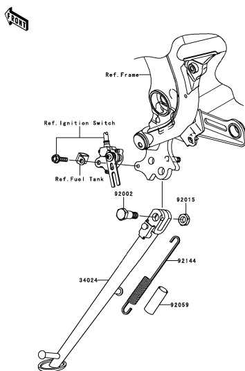
E-12 Stand(s)
