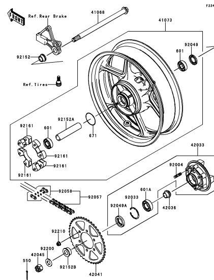
E-14 Rear Hub
