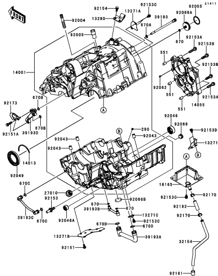
C-4 Crankcase(1/2)
