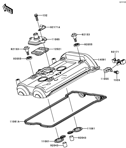
B-4 Cylinder Head Cover
