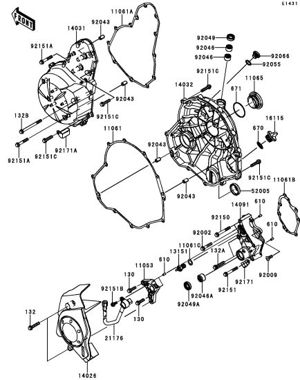
C-7 Engine Cover(s)
