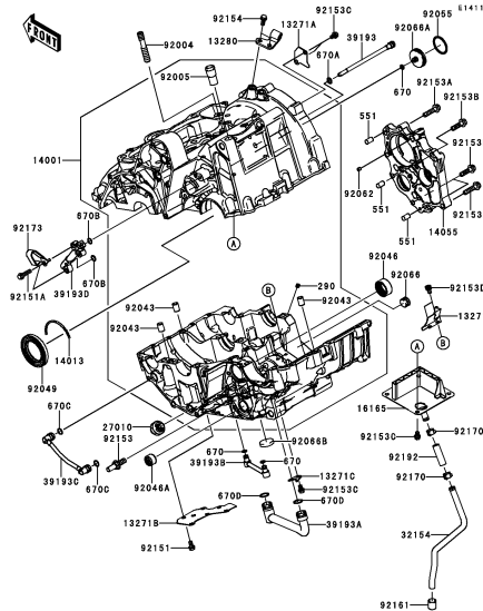
C-5 Crankcase(2/2)
