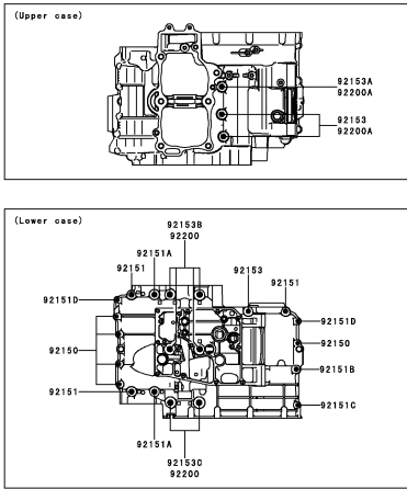
C-6 Crankcase Bolt Pattern
