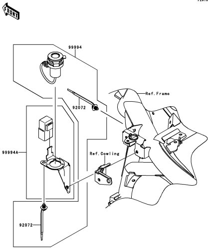
H-3 Accessory(DC12V Socket)
