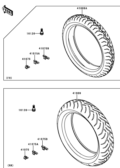
E-12 Tires
