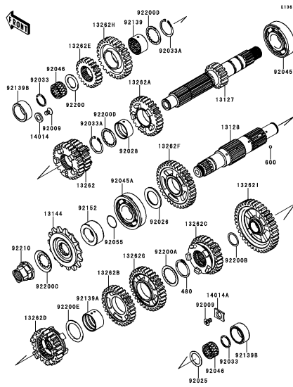
B-13 Transmission
