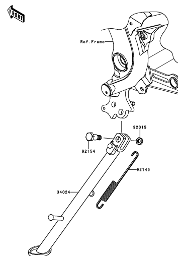
E-11 Stand(s)
