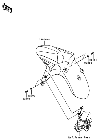
E-9 Front Fender(s)
