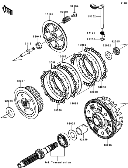
B-12 Clutch
