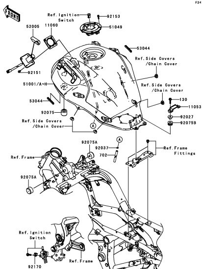
G-3 Fuel Tank(B7F/B8F)
