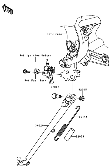
E-12 Stand(s)
