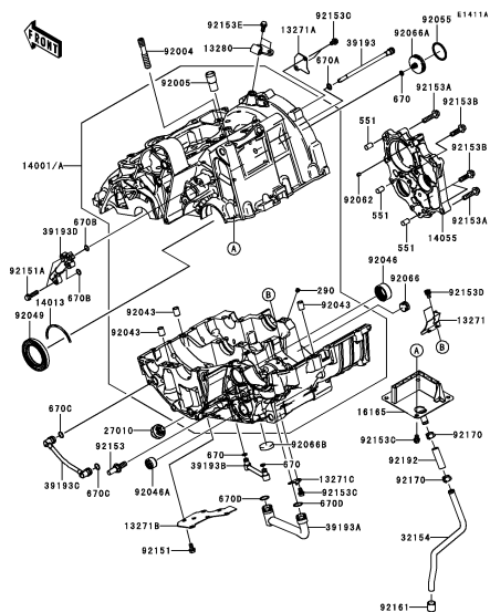
C-6 Crankcase(1/2)(ER650AE057324~)
