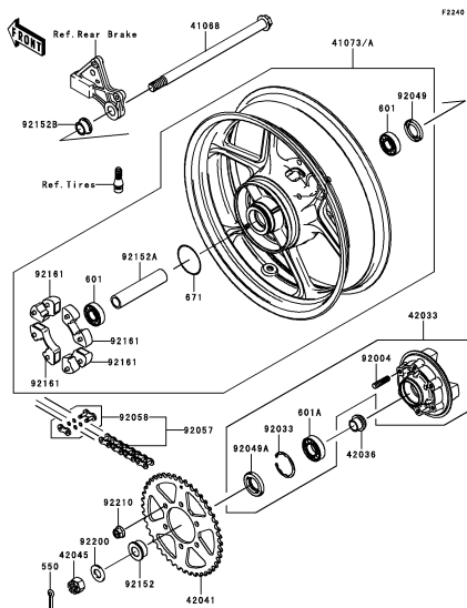
F-3 Rear Hub
