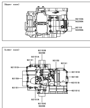
C-9 Crankcase Bolt Pattern
