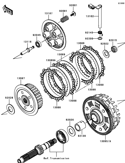
B-12 Clutch
