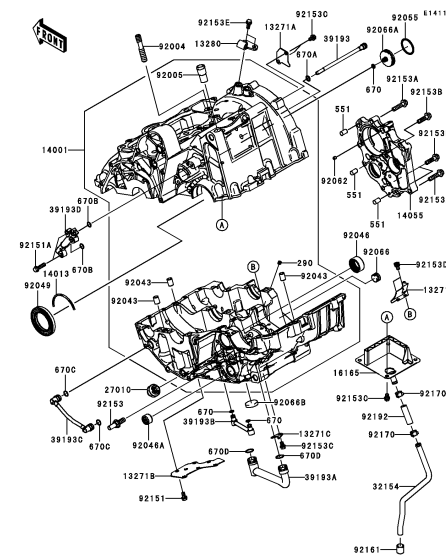
C-5 Crankcase(2/2)(~ER650AE057323)
