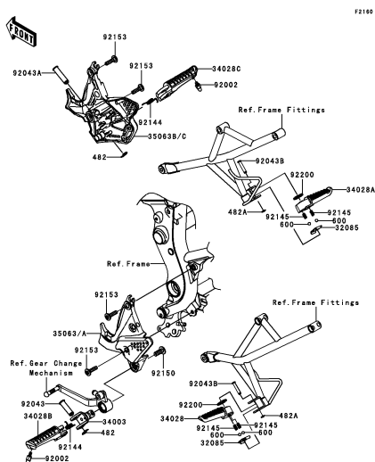
E-9 Footrests
