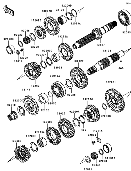
B-13 Transmission
