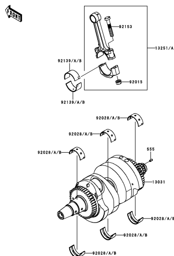
B-10 Crankshaft
