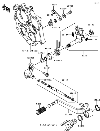
C-3 Gear Change Mechanism
