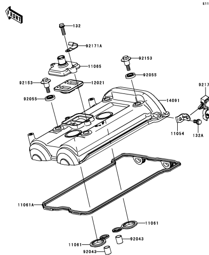
B-4 Cylinder Head Cover
