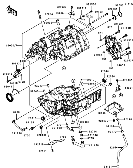
C-7 Crankcase(2/2)(ER650AE057324~)
