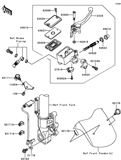
F-6 Front Master Cylinder(B7F/B8F)
