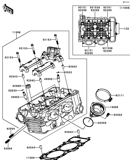
B-3 Cylinder Head
