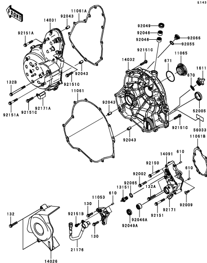
C-10 Engine Cover(s)
