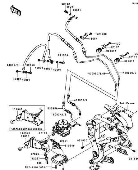
F-5 Brake Piping
