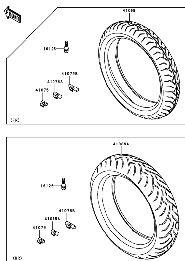
E-13 Tires
