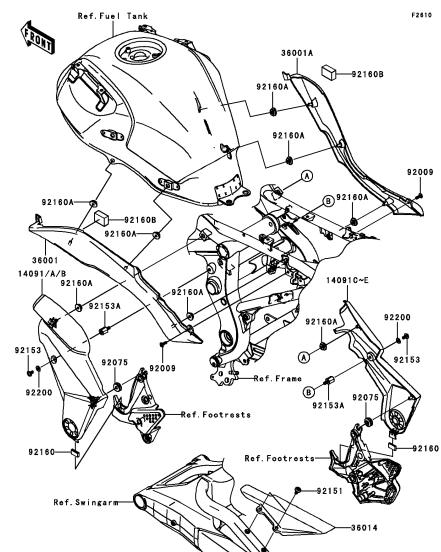
G-8 Side Covers/Chain Cover
