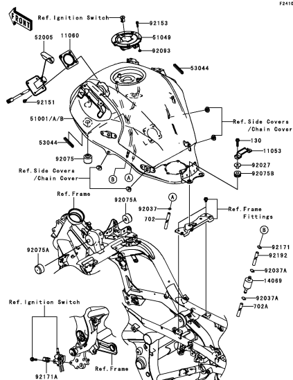
G-4 Fuel Tank(B9F)
