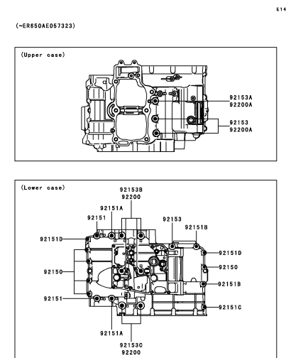
C-5 Crankcase(2/2)(~ER650AE057323)
