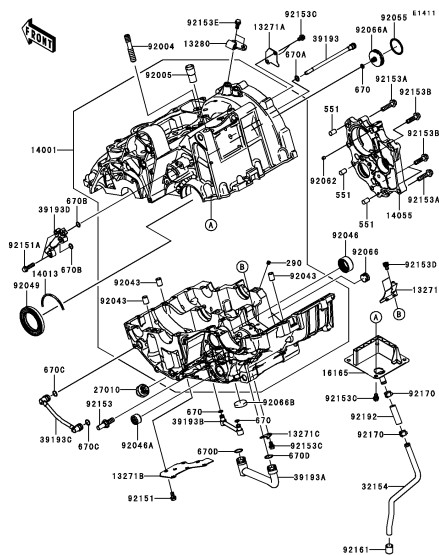
C-4 Crankcase(1/2)(~ER650AE057323)
