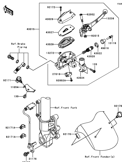
F-7 Front Master Cylinder(B9F)
