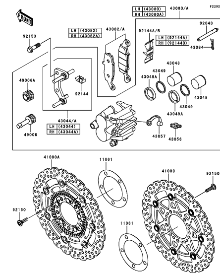
F-8 Front Brake(B7F/B8F)
