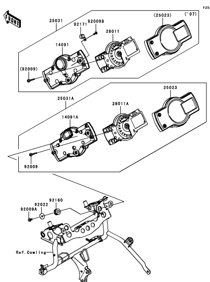
G-6 Meter(s)
