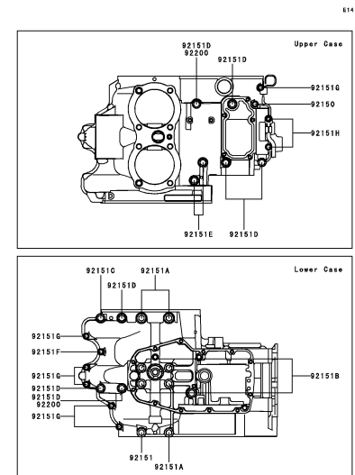
C-8 Crankcase Bolt Pattern
