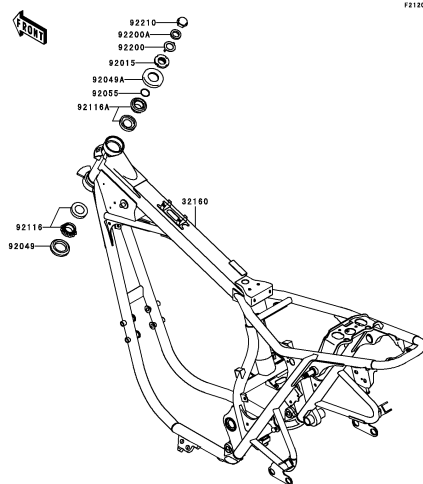
E-3 Frame
