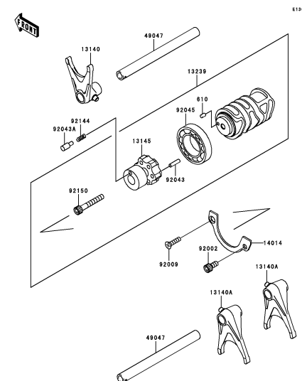
C-5 Gear Change Drum/Shift Fork(s)
