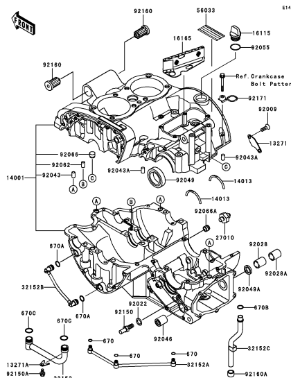
C-7 Crankcase
