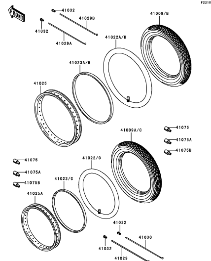
E-11 Tires
