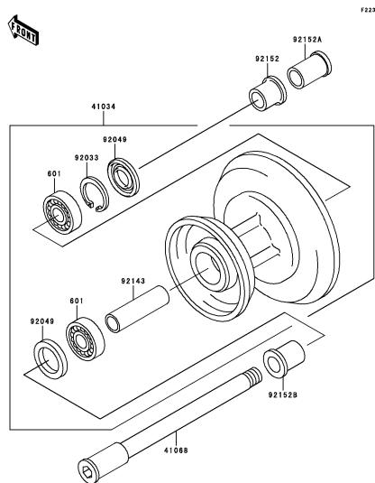
E-12 Front Hub
