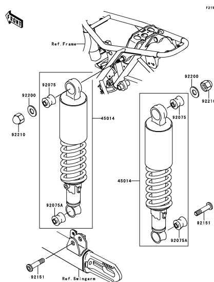
E-7 Suspension/Shock Absorber
