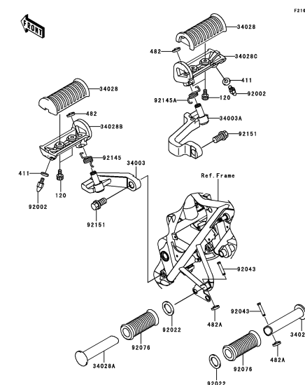
E-8 Footrests
