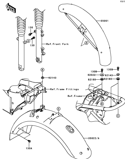
E-9 Fenders
