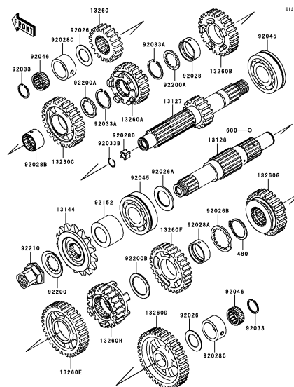
C-4 Transmission
