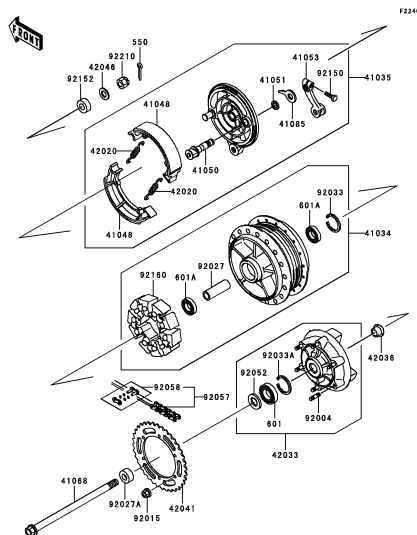
E-13 Rear Hub
