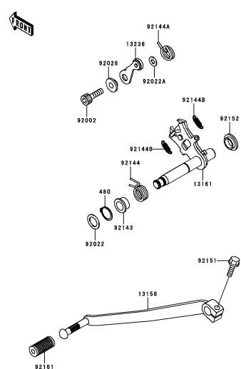
C-6 Gear Change Mechanism
