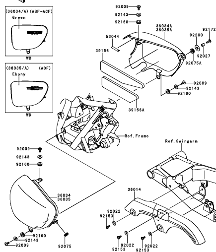
F-12 Side Covers/Chain Cover(ABF~ADF)
