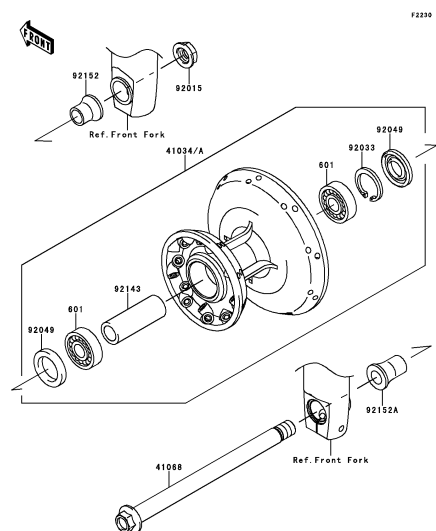
E-12 Front Hub
