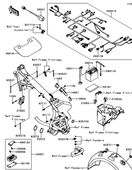
G-5 Chassis Electrical Equipment
