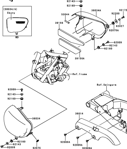
F-13 Side Covers/Chain Cover(ADFA)
