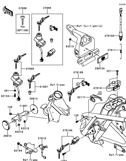
G-6 Ignition Switch
