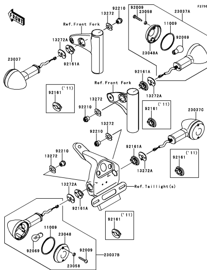
G-4 Turn Signals
