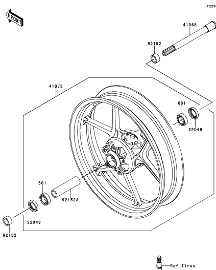
E-13 Front Wheel
