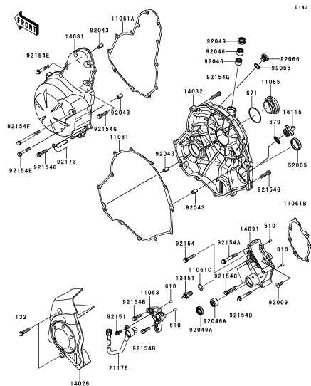
C-7 Engine Cover(s)
