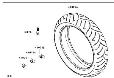
E-12 Tires
