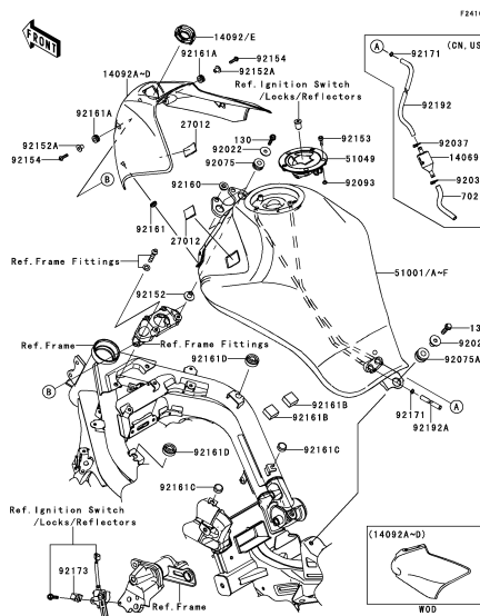
F-10 Fuel Tank(1/2)
