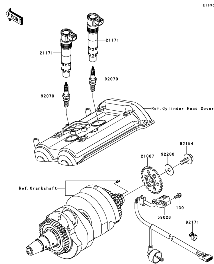
D-3 Ignition System
