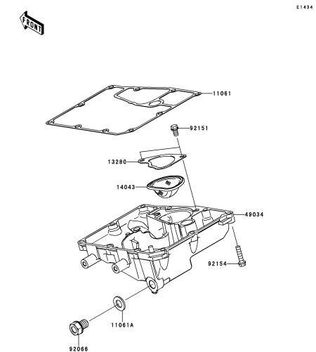
C-5 Crankcase(2/2)
