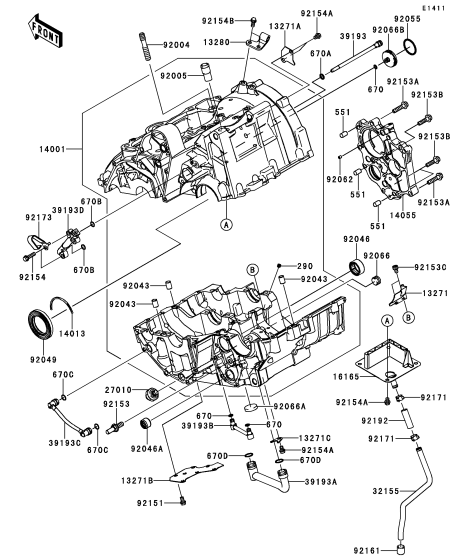
C-5 Crankcase(2/2)
