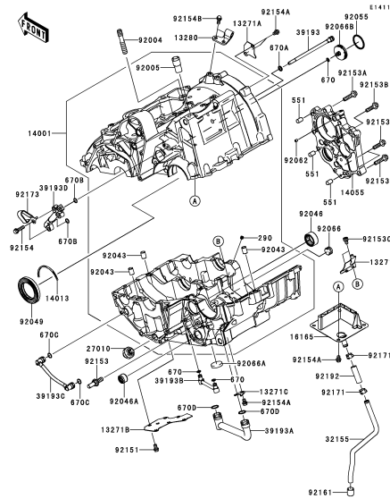
C-4 Crankcase(1/2)
