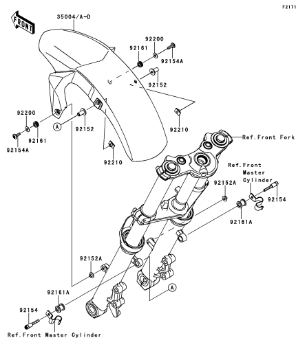
E-9 Front Fender(s)
