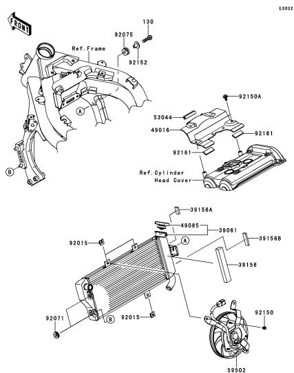
D-6 Radiator
