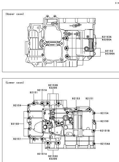
C-6 Crankcase Bolt Pattern
