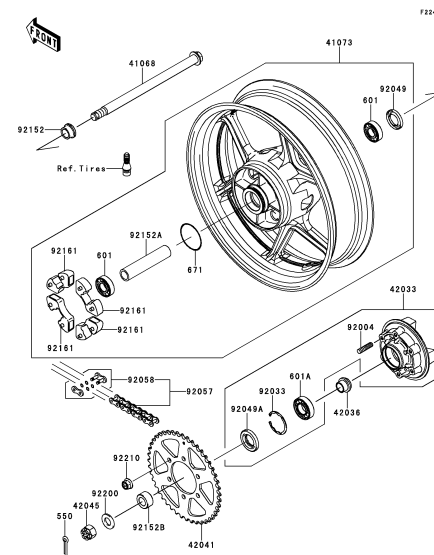
E-14 Rear Wheel/Chain
