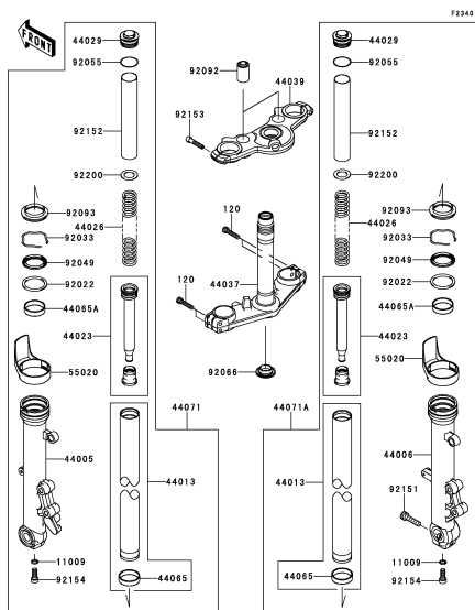
F-9 Front Fork
