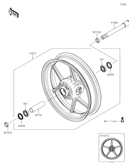
E-13 Front Hub
