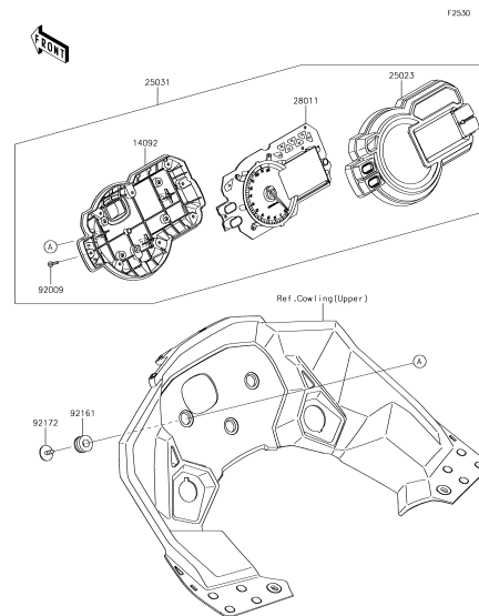
F-13 Meter(s)
