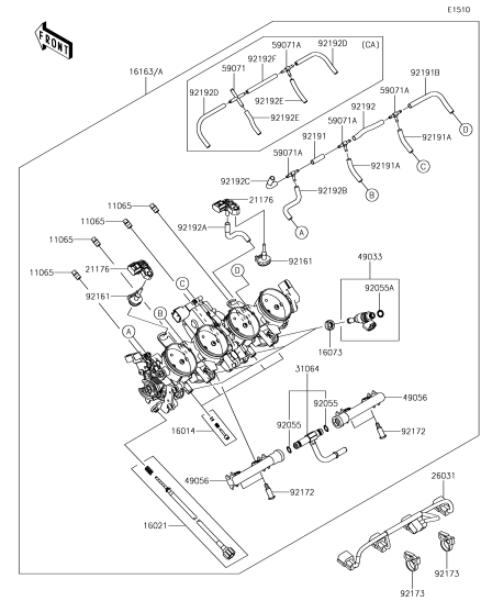
C-8 Throttle
