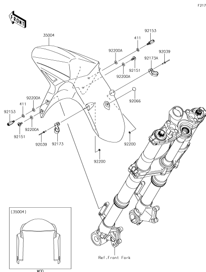
E-9 Front Fender(s)
