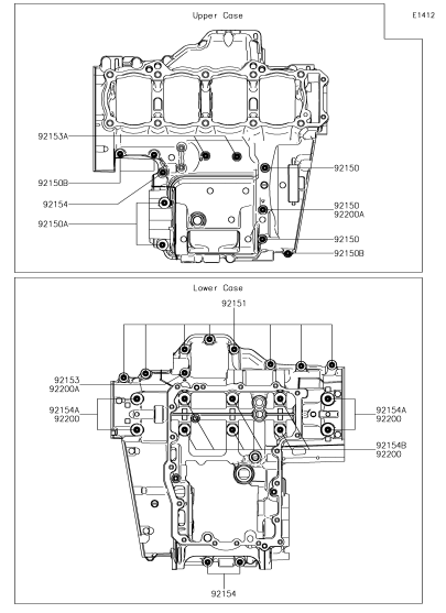
C-5 Crankcase Bolt Pattern
