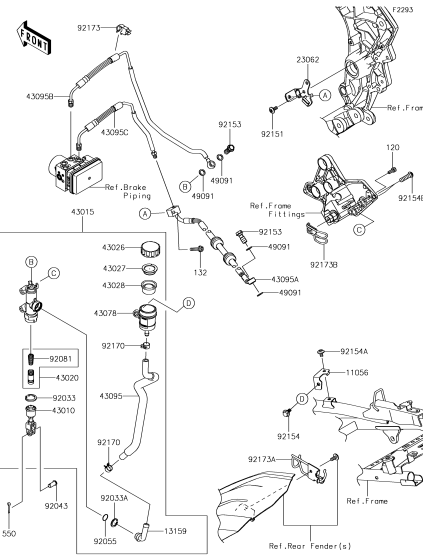
F-7 Rear Master Cylinder
