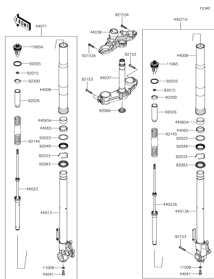
F-10 Front Fork
