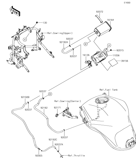
C-11 Fuel Evaporative System(CA)
