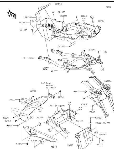
E-10 Rear Fender(s)
