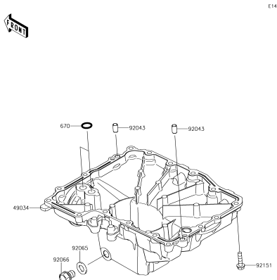
C-4 Crankcase
