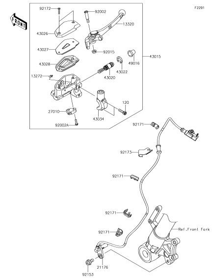
F-5 Front Master Cylinder
