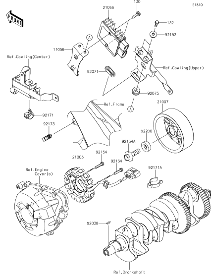
C-13 Generator
