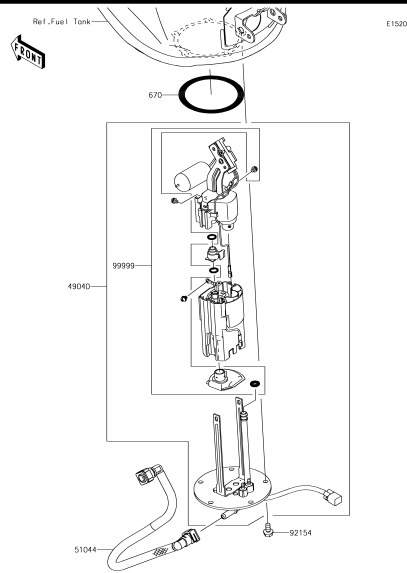
C-9 Fuel Pump
