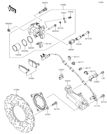
F-8 Rear Brake
