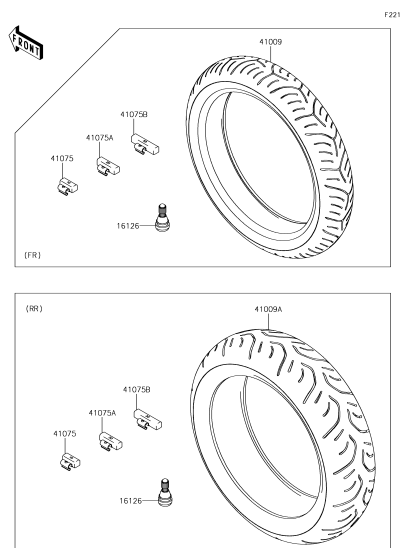
E-12 Wheels/Tires
