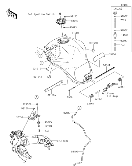
F-11 Fuel Tank
