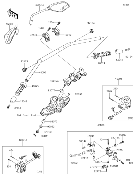
F-9 Handlebar
