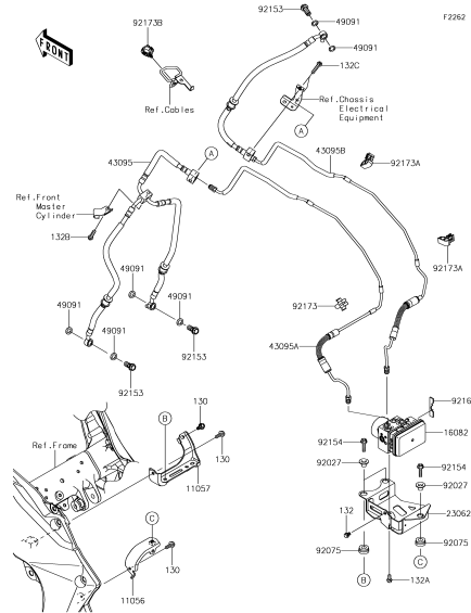
F-4 Brake Piping
