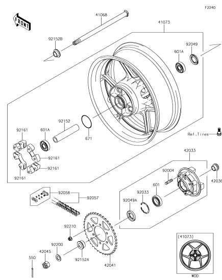
E-14 Rear Hub
