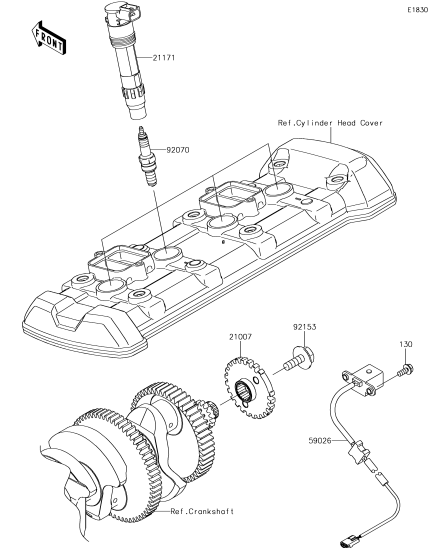
C-14 Ignition System
