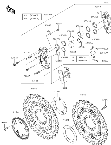
F-6 Front Brake
