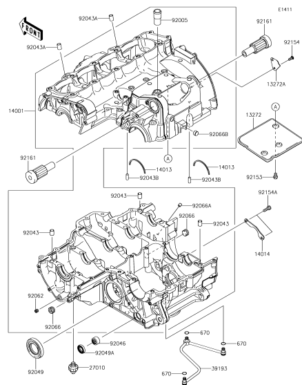
C-4 Crankcase
