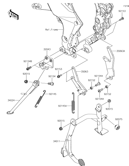
E-11 Stand(s)
