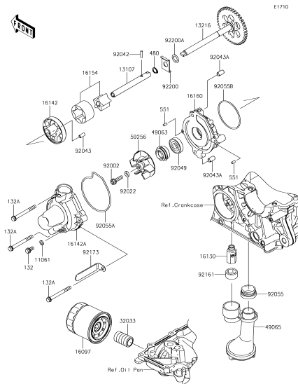
C-12 Oil Pump
