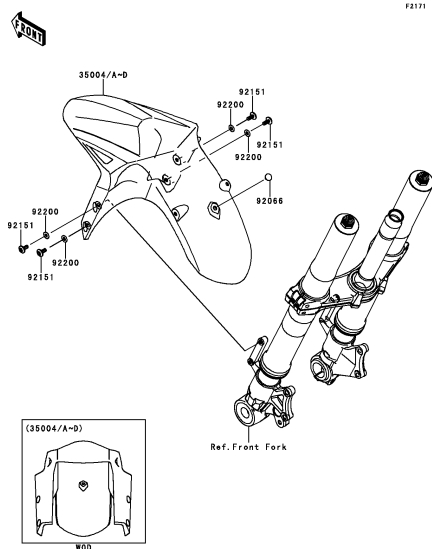
E-9 Front Fender(s)
