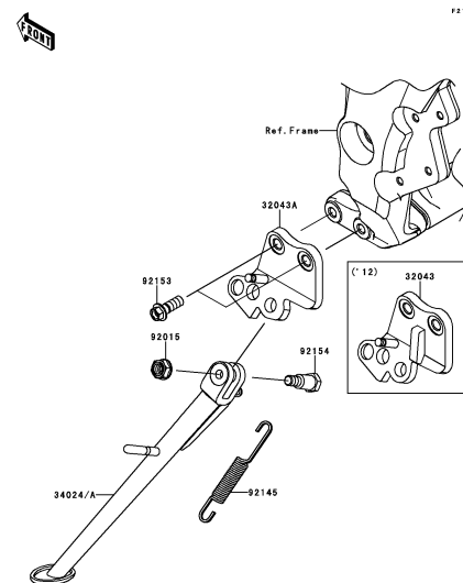
E-11 Stand(s)
