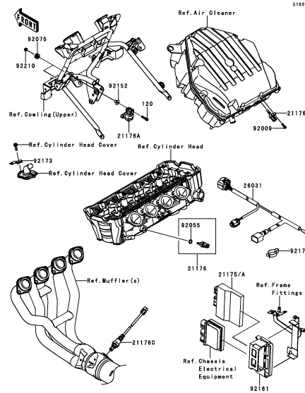
C-10 Fuel Injection
