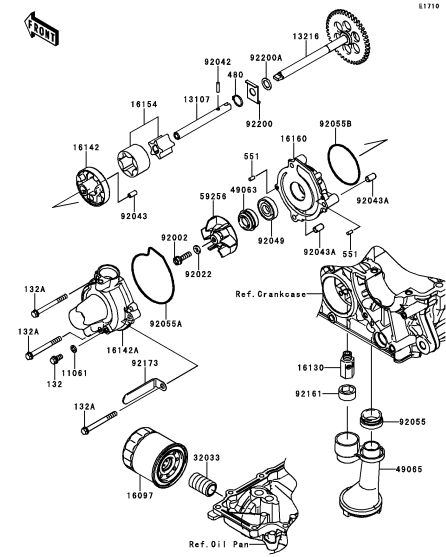
C-11 Oil Pump
