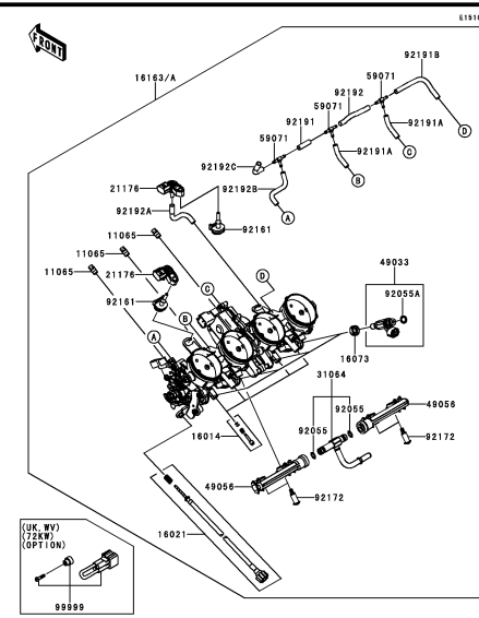
C-8 Throttle
