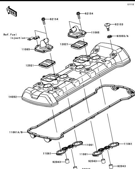
B-4 Cylinder Head Cover
