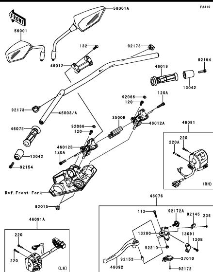
F-9 Handlebar
