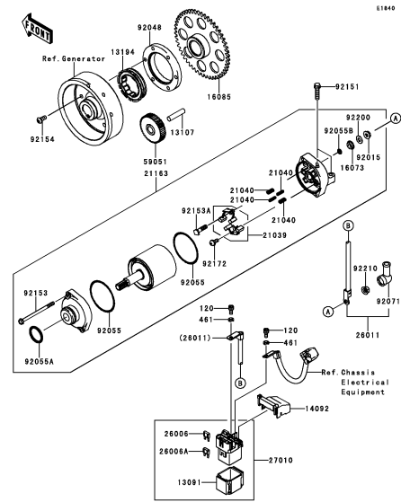
C-14 Starter Motor
