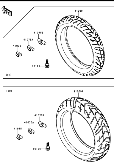
E-12 Tires
