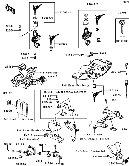
G-9 Ignition Switch(1/2)
