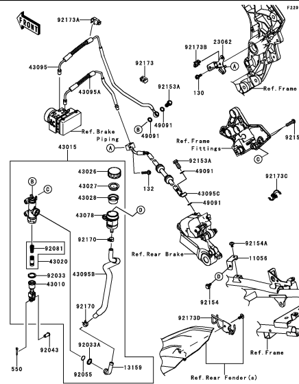
F-7 Rear Master Cylinder
