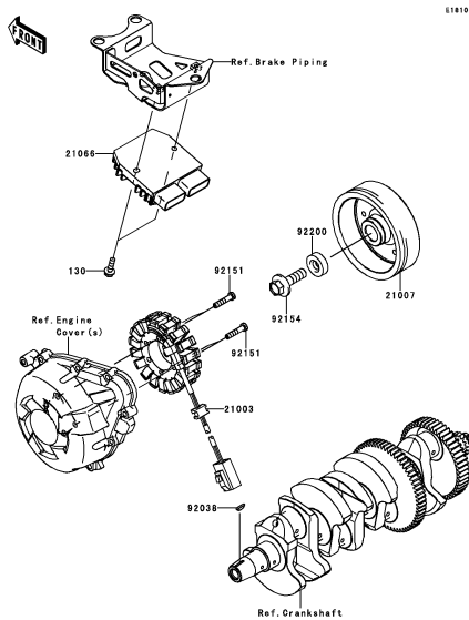
C-12 Generator
