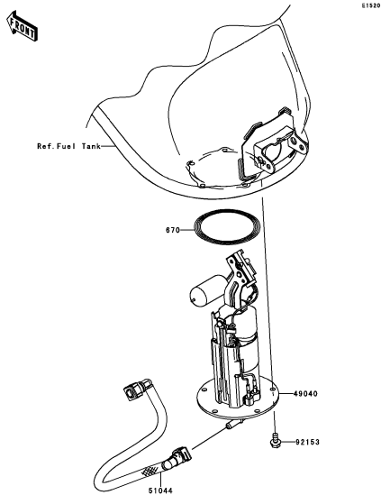
C-9 Fuel Pump
