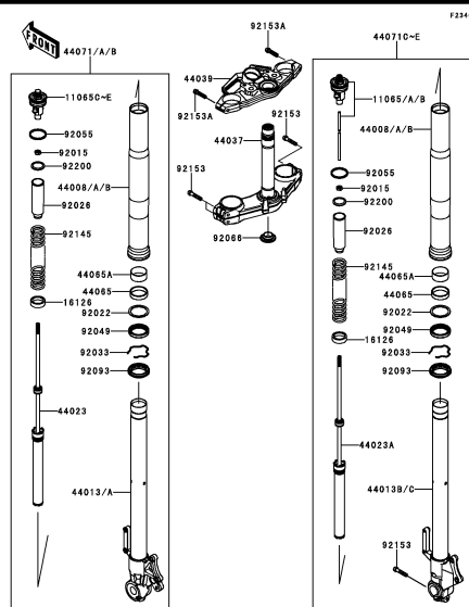
F-10 Front Fork
