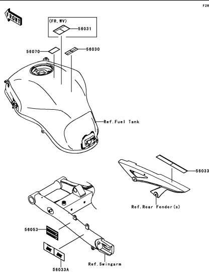
G-12 Labels(ACF)
