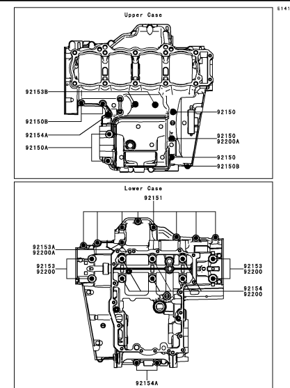
C-5 Crankcase Bolt Pattern
