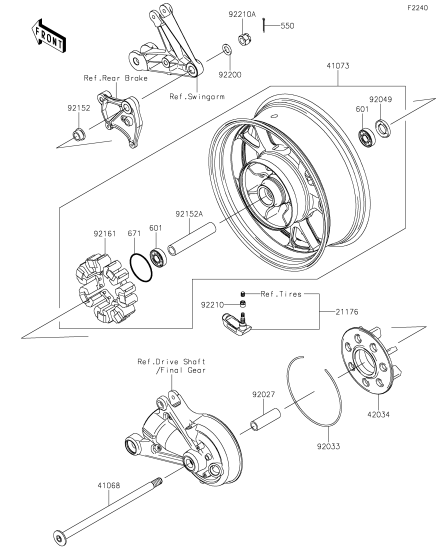
F-5 Rear Wheel/Chain
