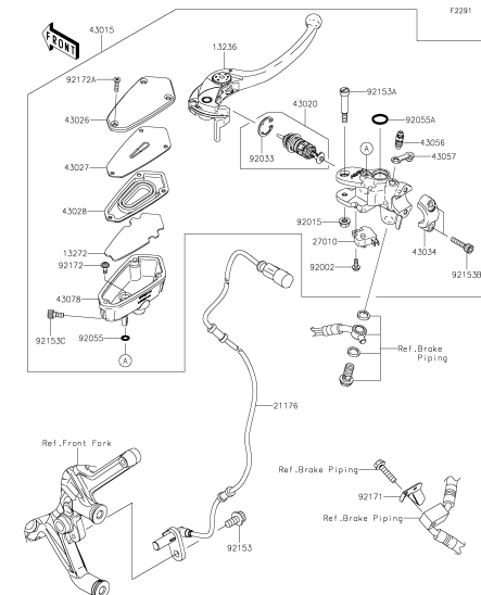
F-8 Front Master Cylinder
