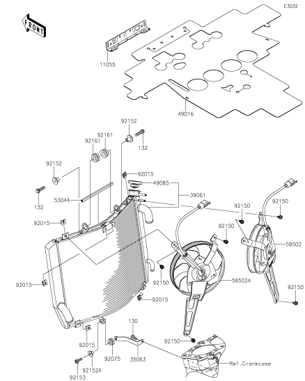
D-5 Radiator
