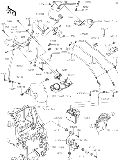
F-7 Brake Piping
