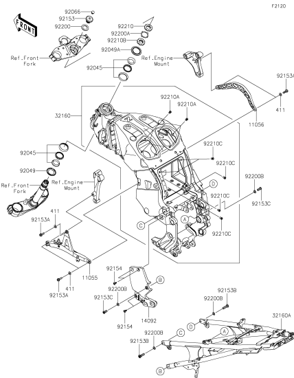
E-3 Frame
