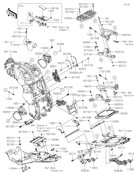
E-6 Frame Fittings(2/2)
