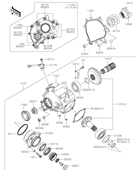
D-8 Front Bevel Gear(1/2)
