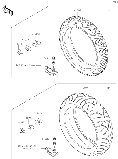
F-3 Tires
