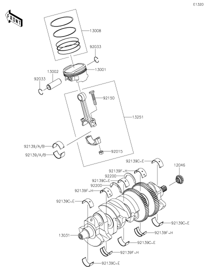
B-10 Crankshaft/Piston(s)
