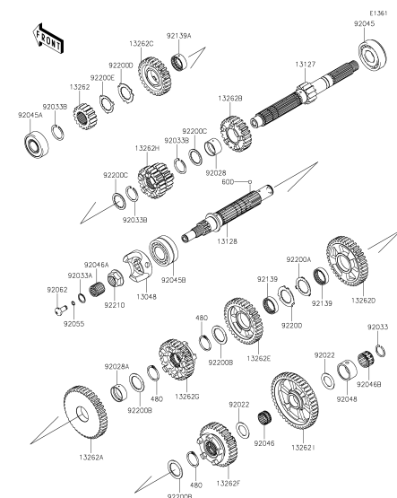
B-14 Transmission
