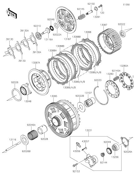
B-12 Clutch(1/2)
