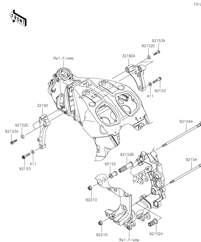
E-4 Engine Mount
