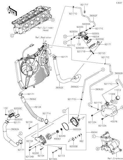
D-7 Water Pipe
