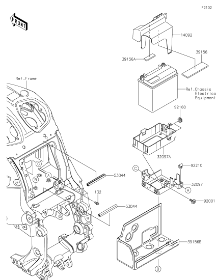
E-7 Battery Case
