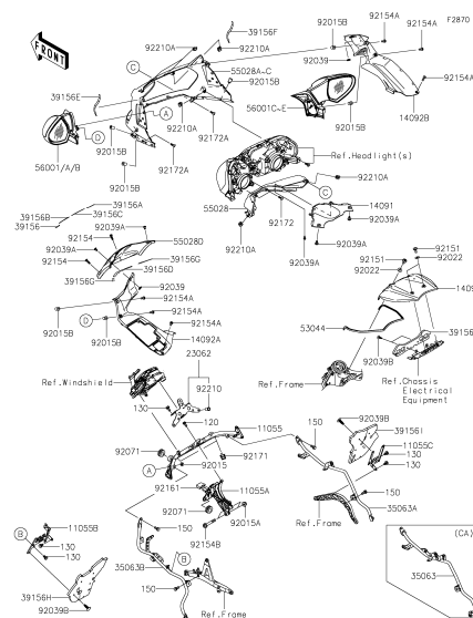
H-13 Cowling(2/2)(Upper)
