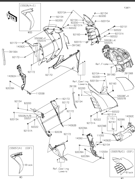
I-3 Cowling(2/2)(Center)
