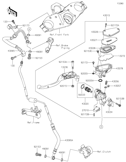
G-3 Clutch Master Cylinder
