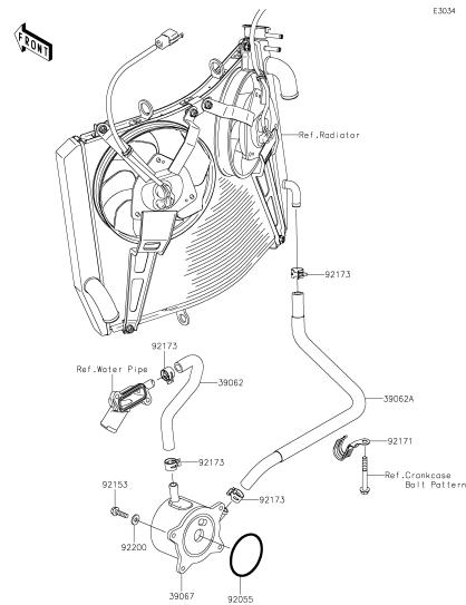
D-6 Oil Cooler
