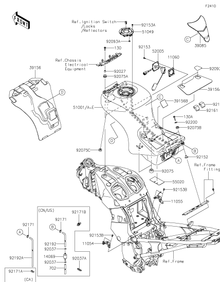
G-4 Fuel Tank(1/2)
