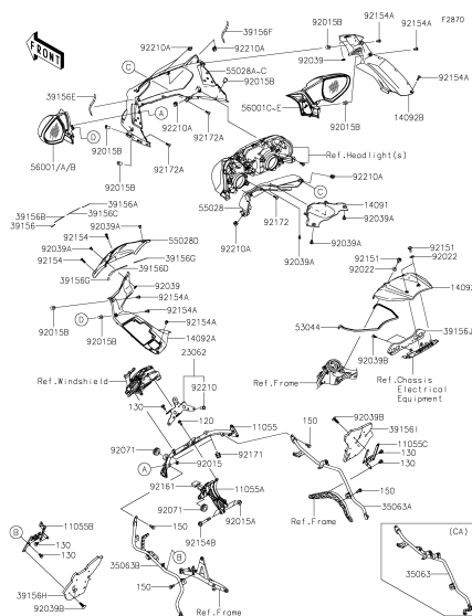
H-12 Cowling(1/2)(Upper)
