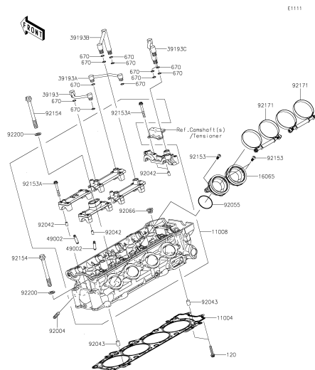
B-3 Cylinder Head
