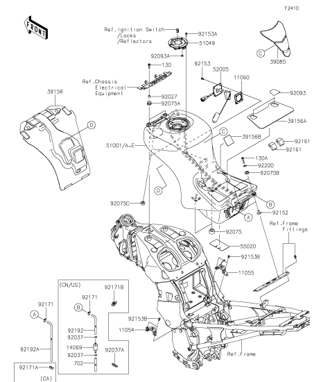
G-5 Fuel Tank(2/2)
