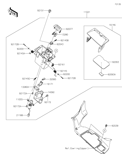
E-8 Front Box
