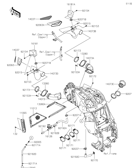
B-5 Air Cleaner
