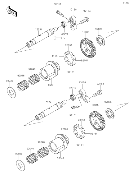
B-11 Balancer
