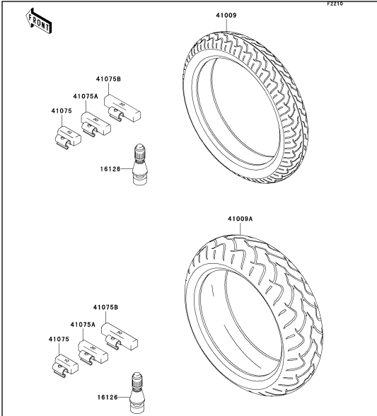
E-11 Tires
