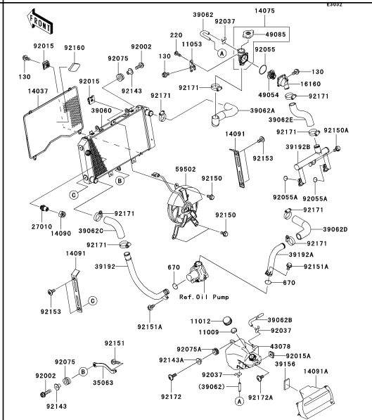
C-14 Radiator(1/2)
