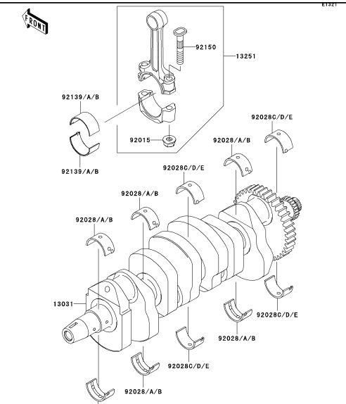
B-10 Crankshaft
