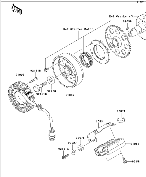
C-11 Generator
