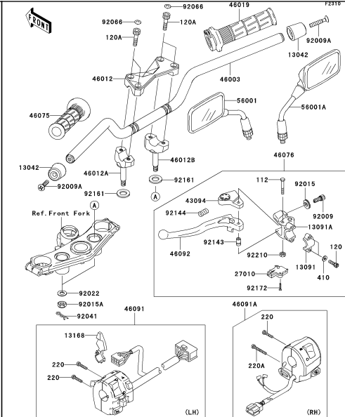
F-8 Handlebar
