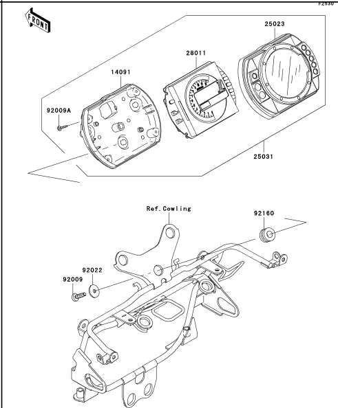
F-13 Meter(s)
