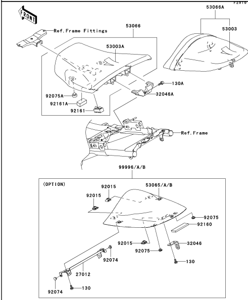
F-12 Seat
