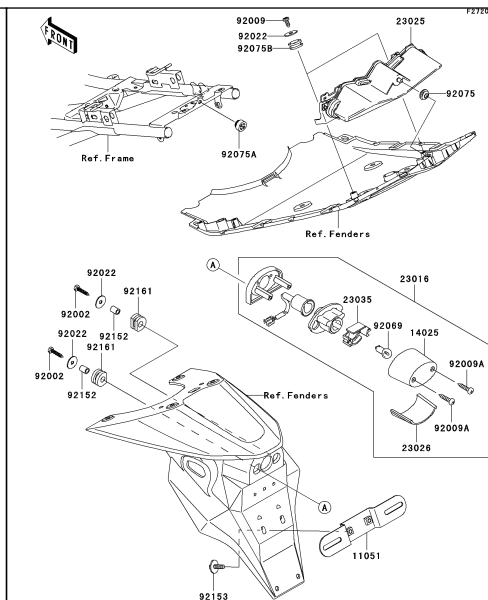
G-5 Taillight(s)
