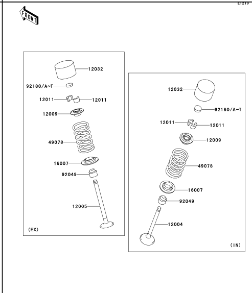
B-8 Valve(s)
