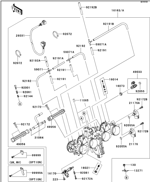
C-7 Throttle
