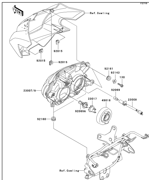
G-4 Headlight(s)
