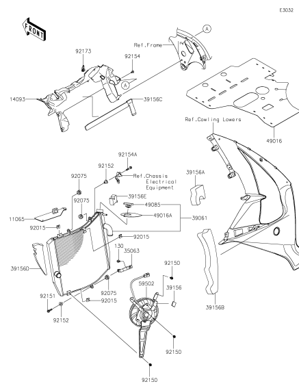
D-7 Radiator
