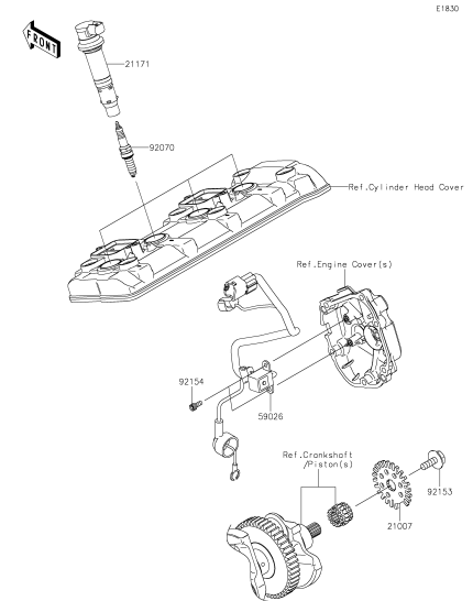
D-5 Ignition System
