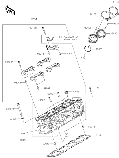
B-3 Cylinder Head
