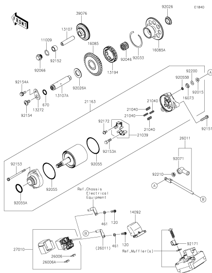
D-6 Starter Motor
