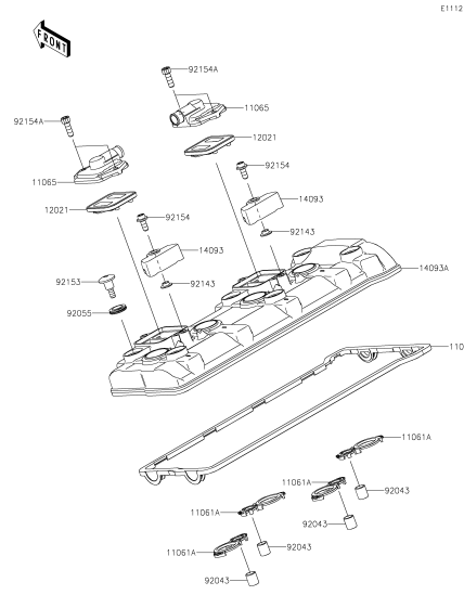
B-4 Cylinder Head Cover
