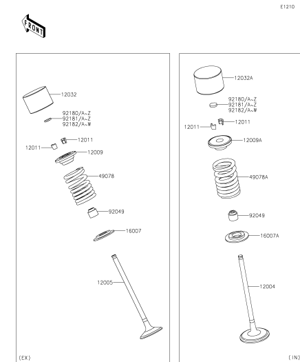
B-8 Valve(s)(1/3)
