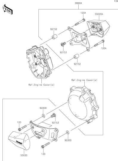
H-4 Accessory(Frame Slider)
