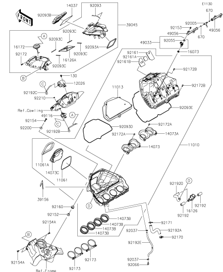
B-5 Air Cleaner(1/2)
