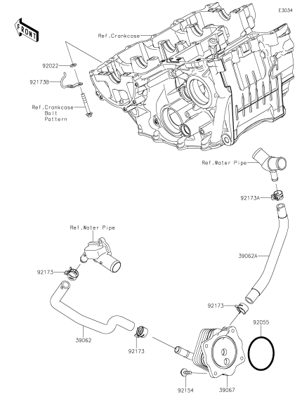
D-8 Oil Cooler
