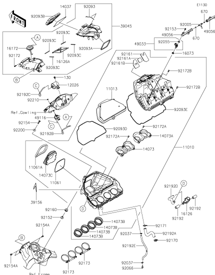
B-6 Air Cleaner(2/2)
