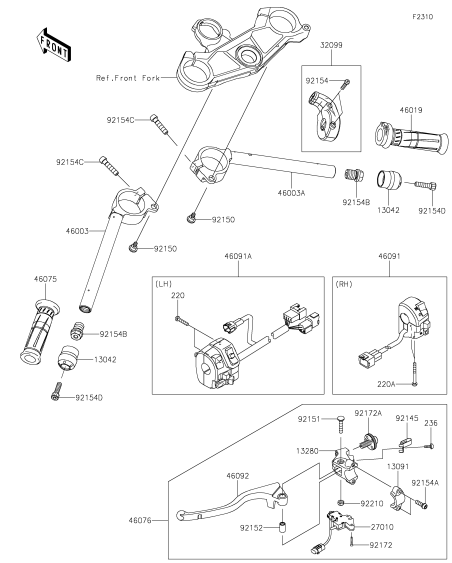
F-8 Handlebar
