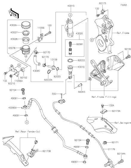
F-6 Rear Master Cylinder
