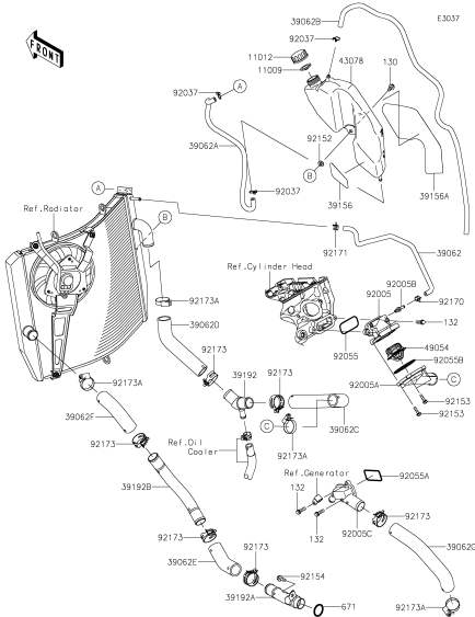
D-9 Water Pipe
