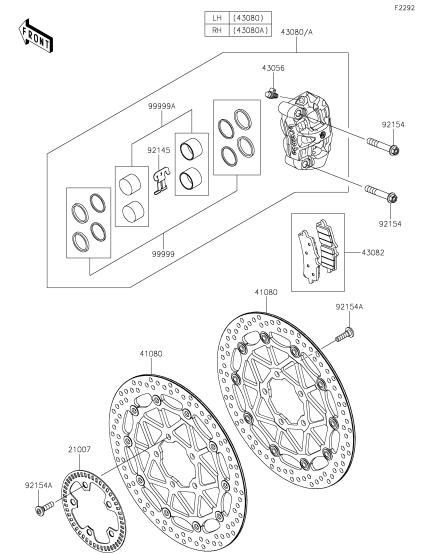
F-5 Front Brake
