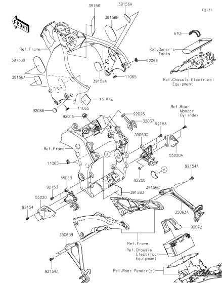
E-5 Frame Fittings
