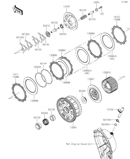
B-14 Clutch
