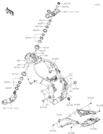
E-3 Frame
