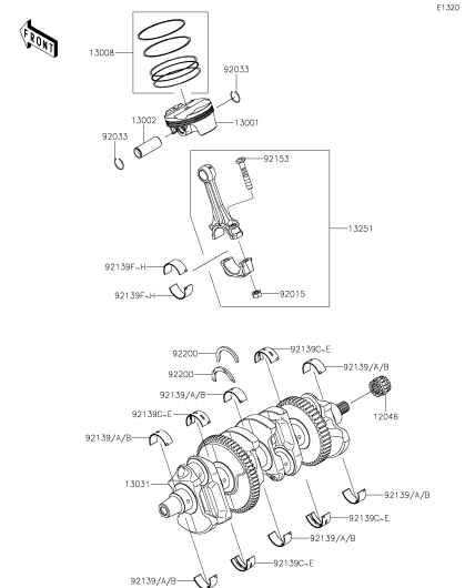
B-12 Crankshaft/Piston(s)
