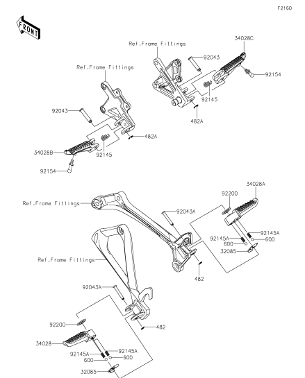
E-8 Footrests
