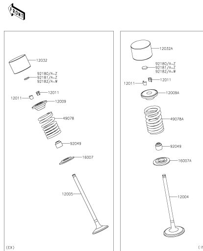
B-10 Valve(s)(3/3)
