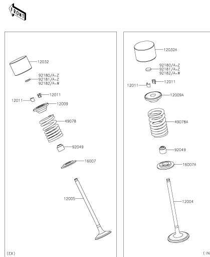
B-9 Valve(s)(2/3)
