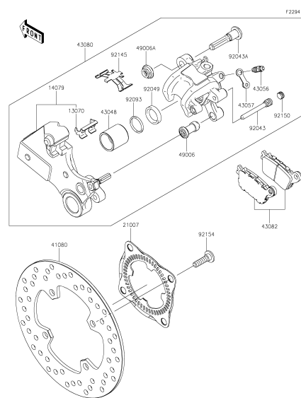
F-7 Rear Brake
