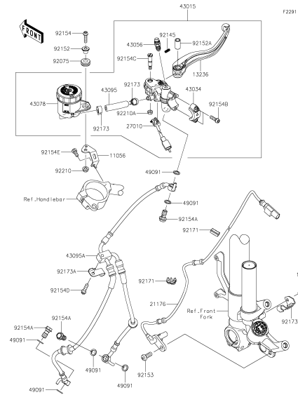
F-4 Front Master Cylinder
