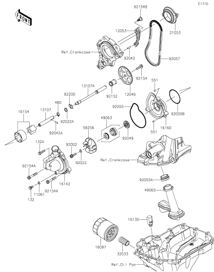
D-3 Oil Pump
