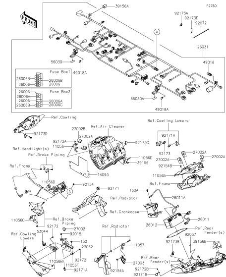
G-11 Chassis Electrical Equipment(2/2)
