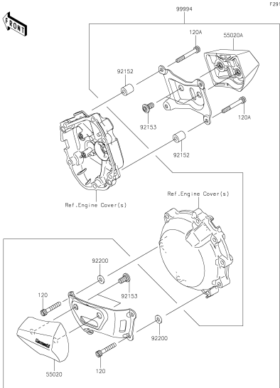
H-9 Accessory(Frame Slider)
