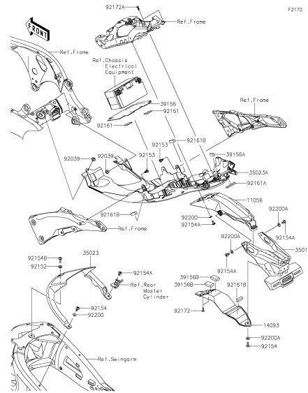
E-10 Rear Fender(s)
