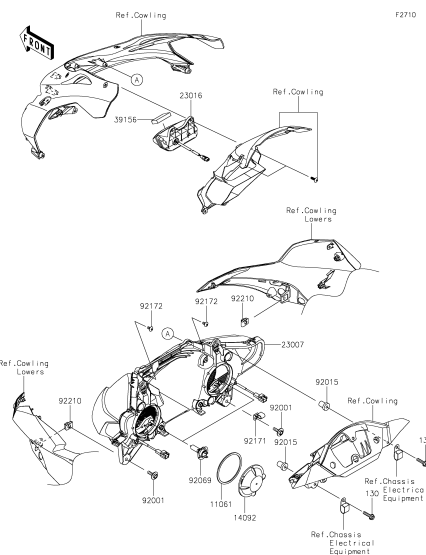
G-7 Headlight(s)
