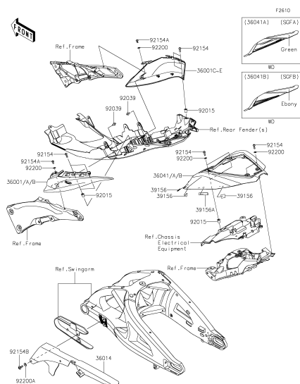
G-6 Side Covers/Chain Cover
