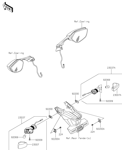
G-9 Turn Signals
