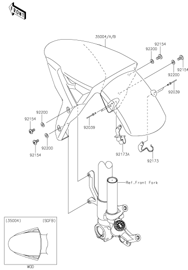
E-9 Front Fender(s)
