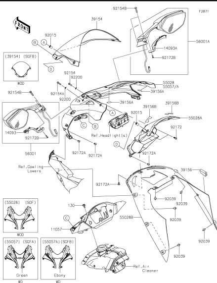
H-6 Cowling
