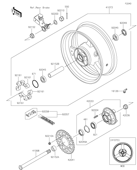
E-14 Rear Hub
