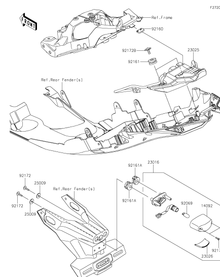
G-8 Taillight(s)
