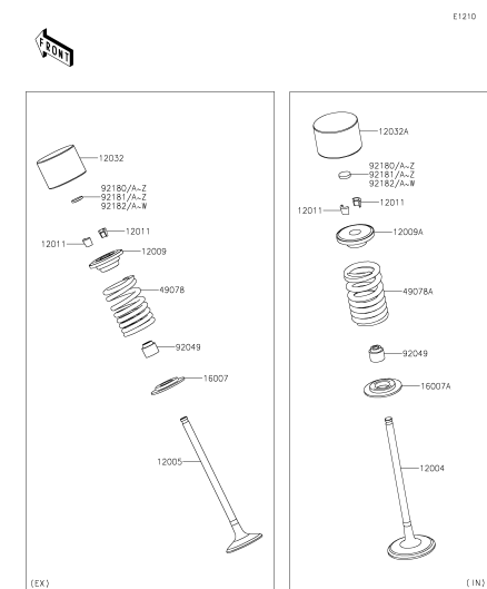
B-8 Valve(s)(1/3)
