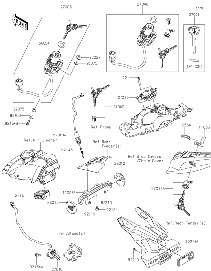
G-12 Ignition Switch
