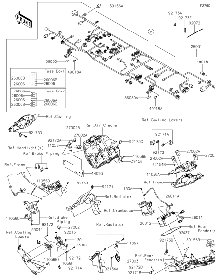
G-10 Chassis Electrical Equipment(1/2)
