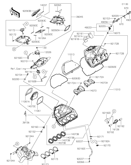
B-5 Air Cleaner(1/2)
