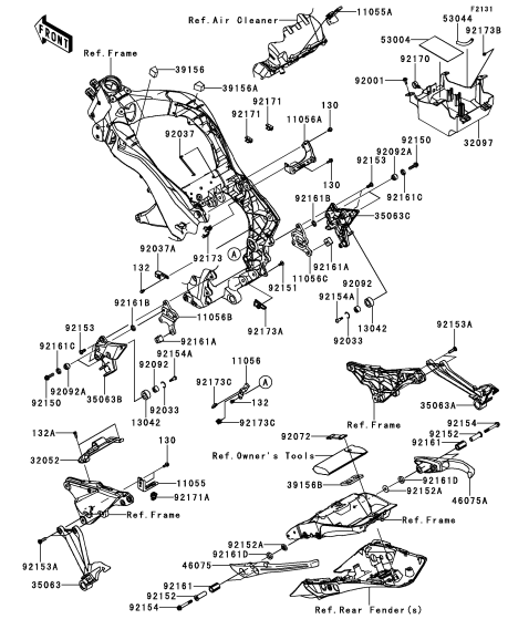
E-5 Frame Fittings(1/2)
