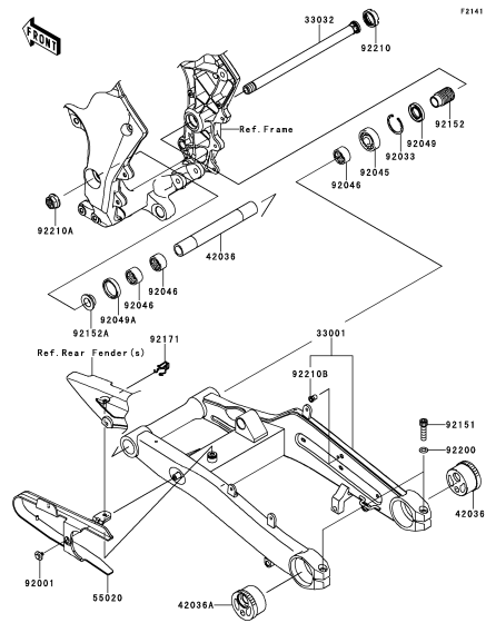
E-7 Swingarm
