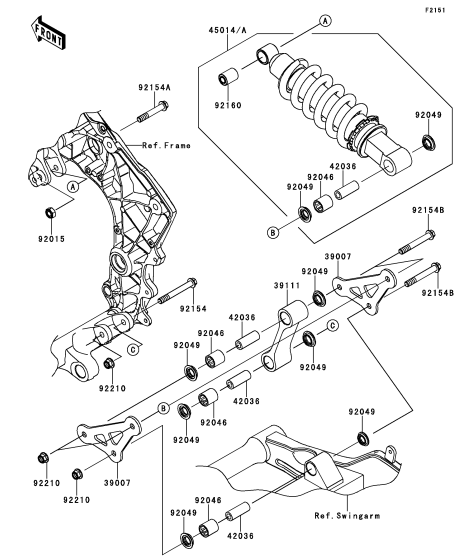
E-8 Suspension/Shock Absorber
