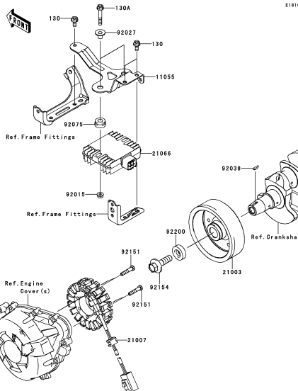
C-13 Generator
