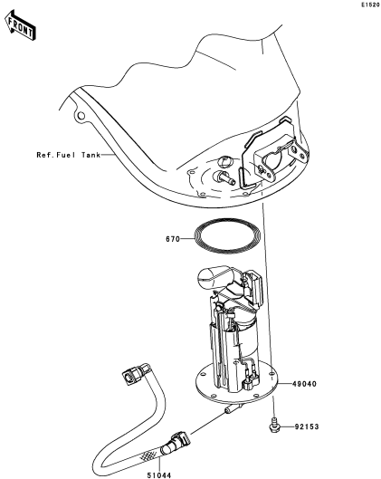
C-9 Fuel Pump
