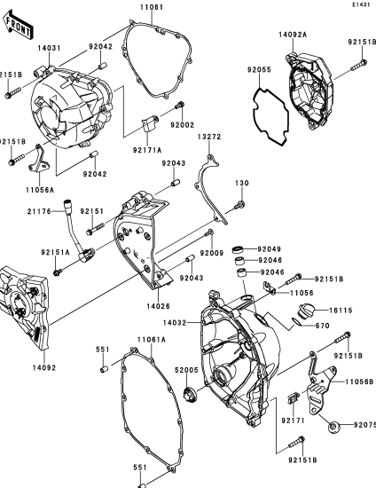
C-6 Engine Cover(s)
