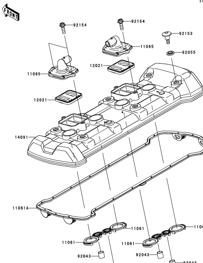
B-4 Cylinder Head Cover
