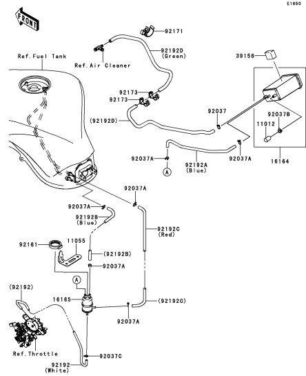
C-11 Fuel Evaporative System(CA)
