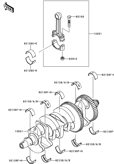
B-10 Crankshaft
