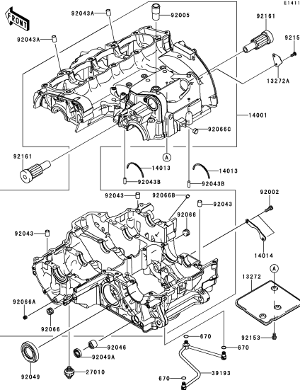
C-4 Crankcase
