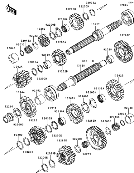
B-13 Transmission
