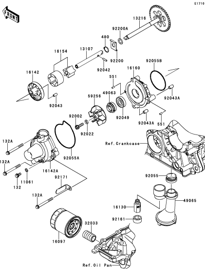
C-12 Oil Pump/Oil Filter
