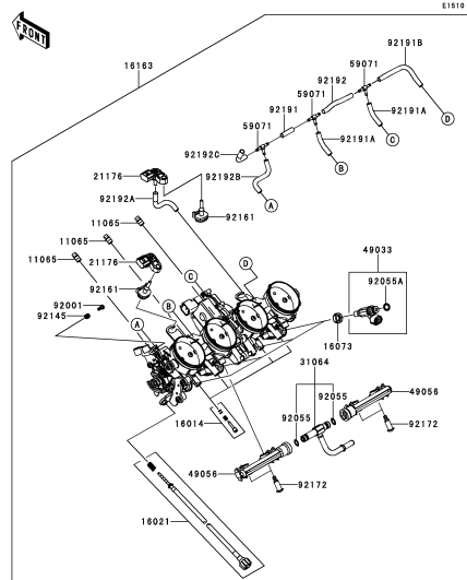
C-8 Throttle
