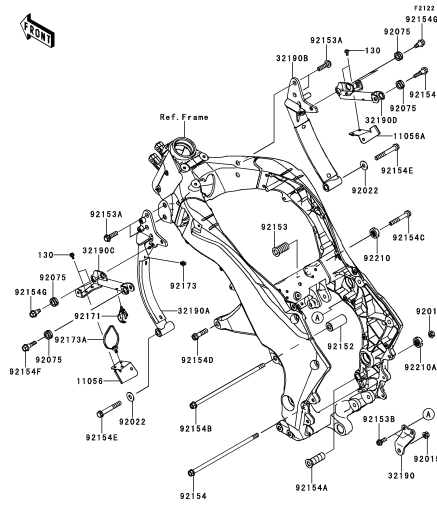
E-4 Engine Mount
