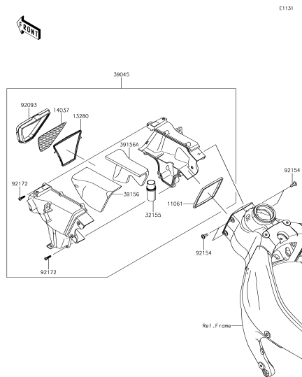
B-6 Air Duct
