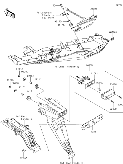
G-7 Taillight(s)
