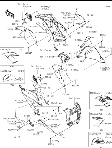
H-7 Cowling Lower (2/2) (FGF/FGFA)
