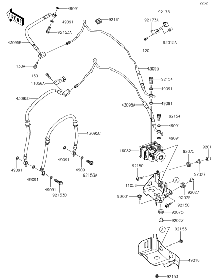
F-4 Brake Piping
