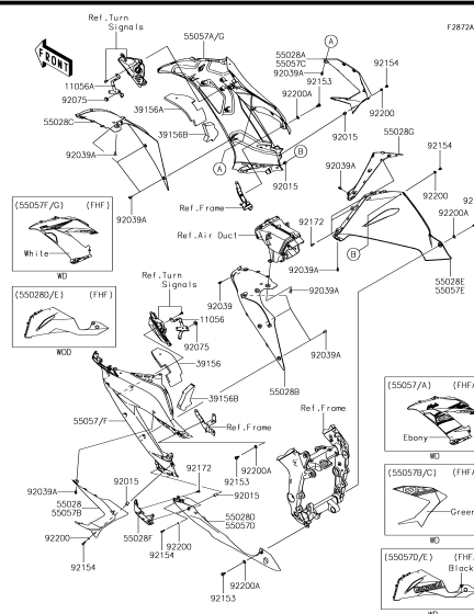
H-8 Cowling Lower (FHF/FHFA)
