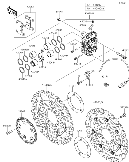
F-6 Front Brake
