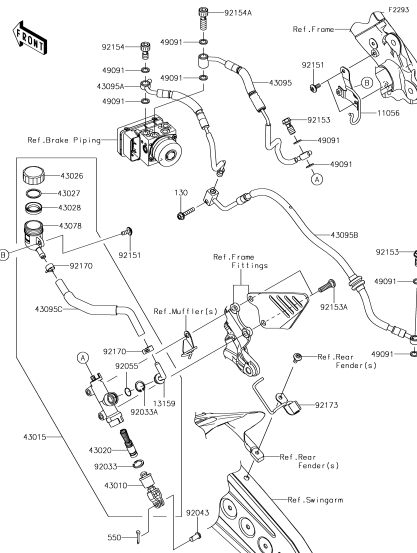
F-7 Rear Master Cylinder
