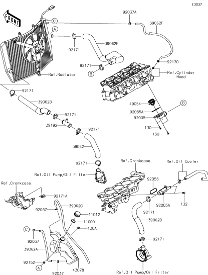
D-9 Water Pipe
