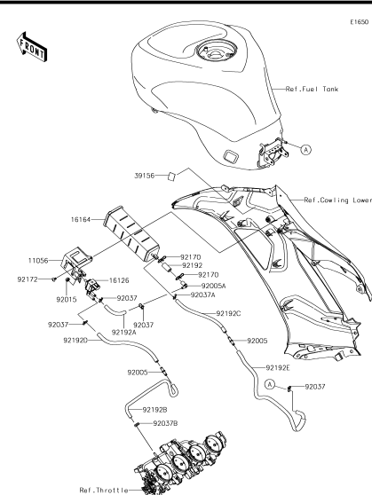
C-14 Fuel Evaporative System(CA)
