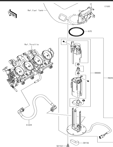
C-12 Fuel Pump
