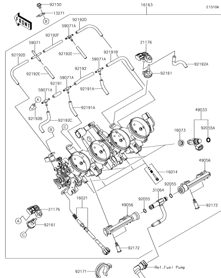
C-10 Throttle(1/2)(CA)
