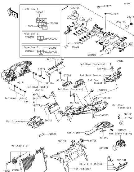
G-9 Chassis Electrical Equipment
