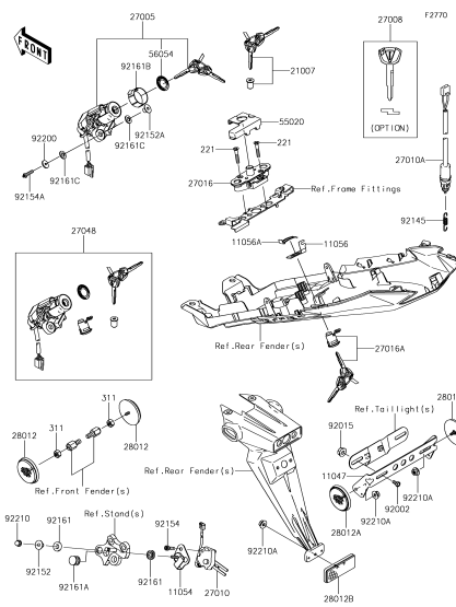
G-10 Ignition Switch/Locks/Reflectors
