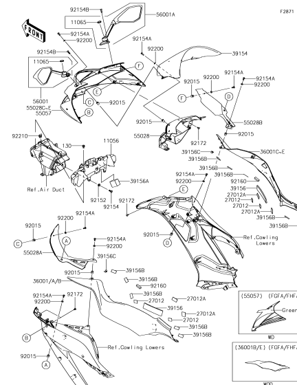
H-5 Cowling
