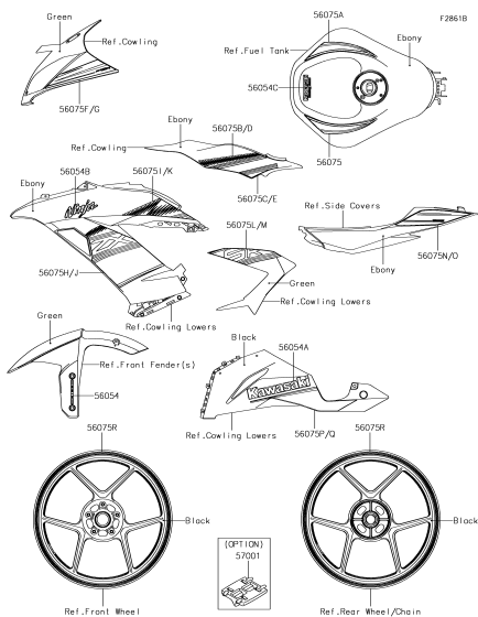
H-3 Decals (Green) (FGFA/FHFA)
