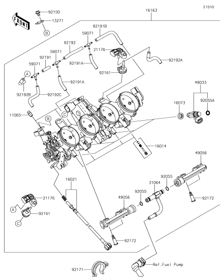
C-9 Throttle(2/2)(CN,US)
