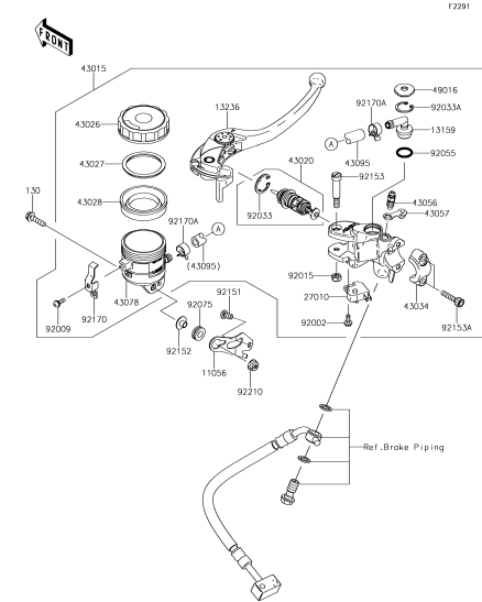
F-5 Front Master Cylinder
