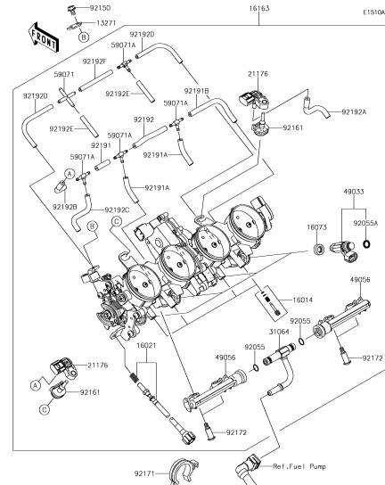
C-11 Throttle(2/2)(CA)
