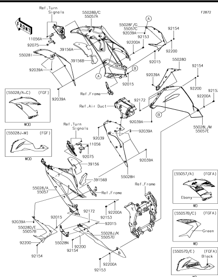
H-6 Cowling Lower (1/2) (FGF/FGFA)
