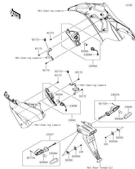
G-8 Turn Signals
