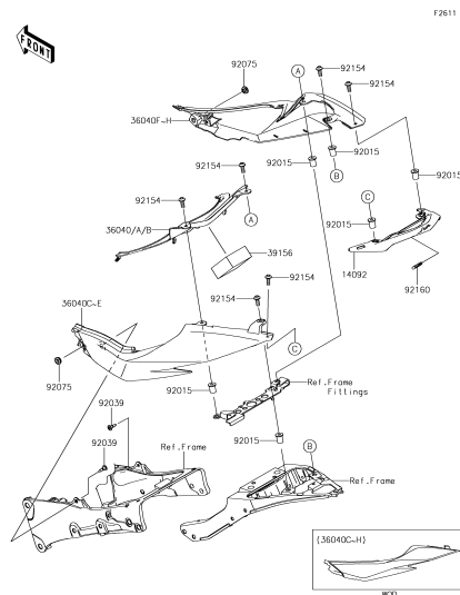
G-4 Side Covers
