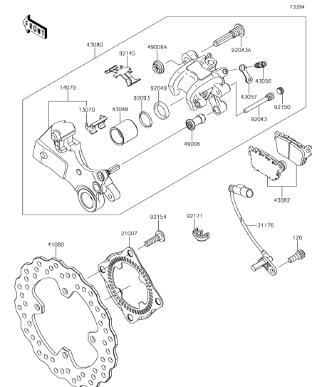
F-8 Rear Brake
