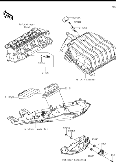
C-13 Fuel Injection
